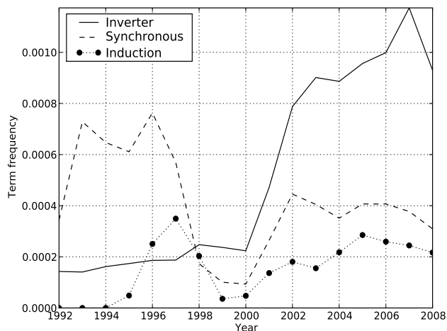
(a) Unnormalized
