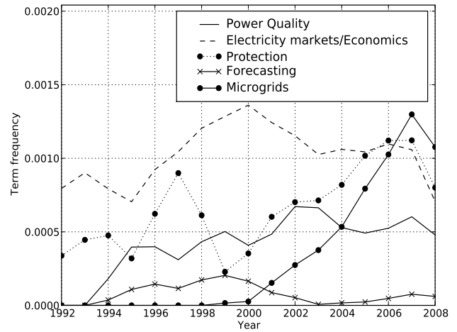
(a) Unnormalized
