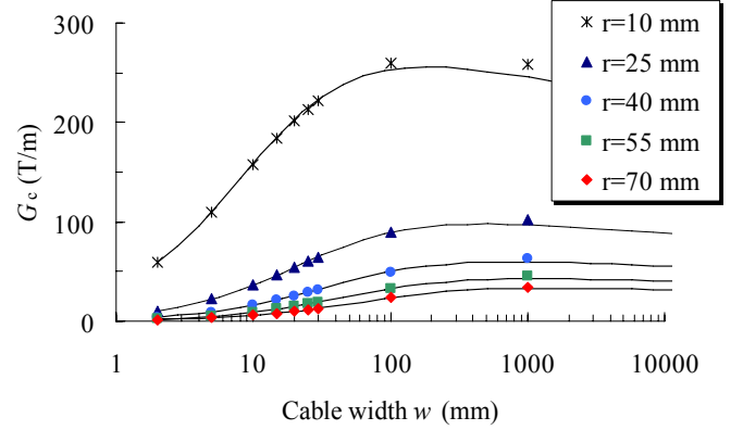
Fig. 6: Critical gradient versus cable width for different apertures: numerical results (dots) and analytical approximation (solid lines) for the cross-quadrupole model, for \kappa=0.33 .
