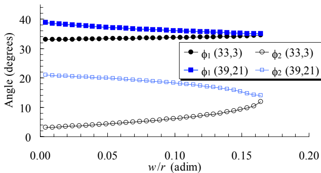
Fig. 31: Two solutions for setting to zero B_6 and B_{10} : angular width of the inner and outer sector \phi_1 and \phi_2 versus ratio w/r .
