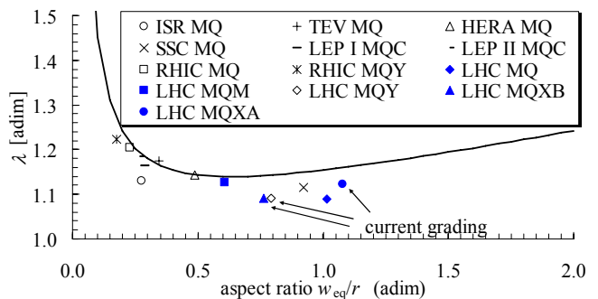
Fig. 25: Ratio \lambda between peak field and current density vs. aspect ratio as defined in Eq. (41): computation for a sector coil (solid line) and values for 13 quadrupoles evaluated without iron (markers).
