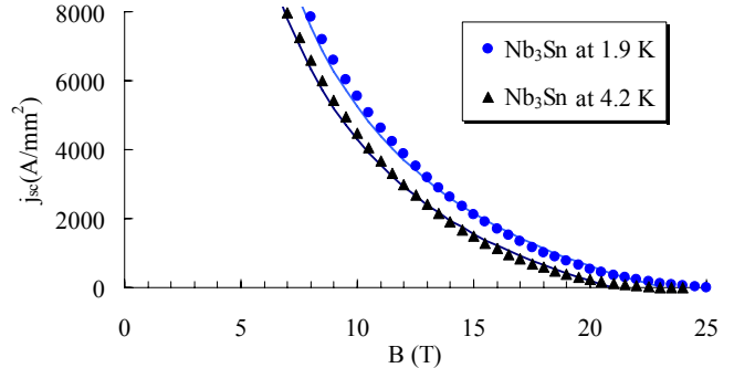
Fig. 28: Critical surface for Nb 3 Sn at 1.9 K and at 4.2 K according to Kramer law (markers), and fit given in Eq. (40) (solid line).
