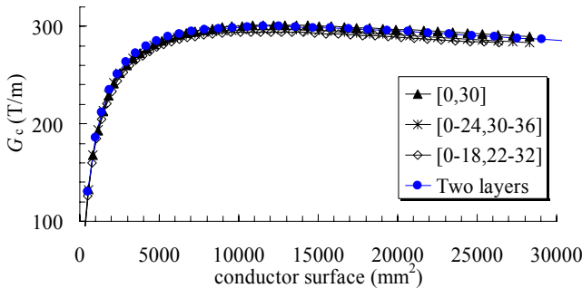
Fig. 12: Numerical evaluation of the critical gradient versus conductor surface for different sector layouts.
