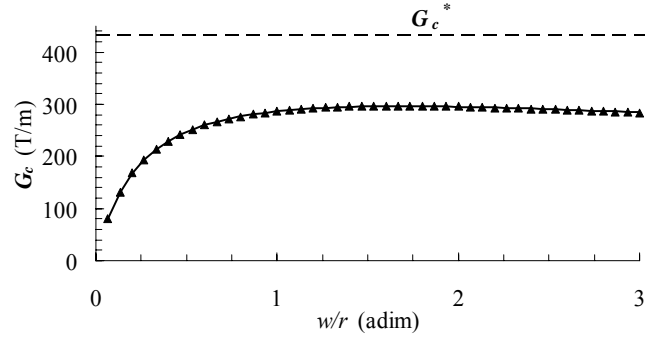
Fig. 13: Critical gradient versus sector width for the [0^\circ\text{-}24^\circ, 30^\circ\text{-}36^\circ] sector: numerical results (markers) and analytical approximation by (37) (solid line).
