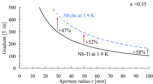
Fig. 27: Maximum critical gradient as a function of aperture radius for Nb-Ti and Nb 3 Sn at 1.9 K for a sector coil of [0°-24°, 30°-36°], \kappa=0.35 .
