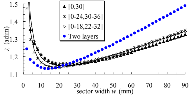
Fig. 10: Numerical evaluation of the function \lambda defined in Eq. (31) versus sector width for different sector layouts, aperture radius of 30 mm, and fitting curves as defined in (32) for the [0^\circ, 30^\circ] and [0^\circ-24^\circ, 30^\circ-36^\circ] design.
