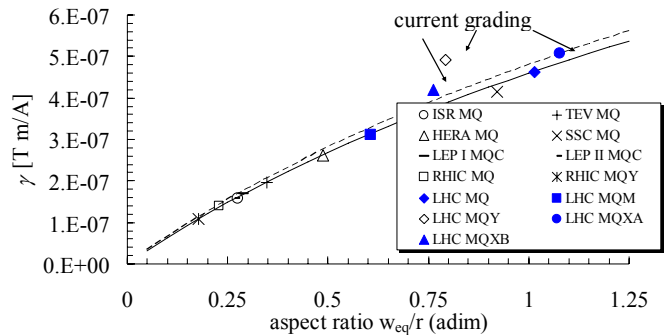
Fig. 24: Parameter \gamma (field gradient per current density) for 13 accelerator quadrupoles without iron (markers) and results for a 30^\circ sector (dashed line) and [0^\circ\text{-}24^\circ, 30^\circ\text{-}36^\circ] sector (solid line) versus aspect ratio as defined in Eq. (41).
