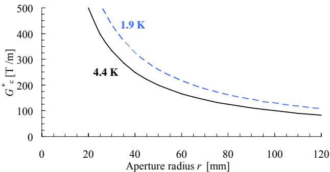
Fig. 4: Theoretical upper bound G_c^* to critical gradient for Nb-Ti as a function of the aperture radius.
