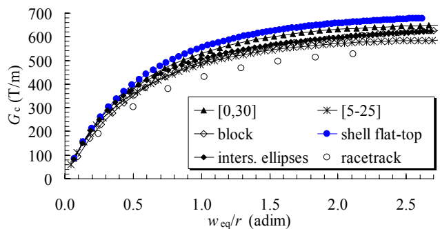
Fig. 21: Numerical evaluation of the critical gradient versus equivalent sector width (41) in six coil layouts with an aperture radius of 10 mm ( \kappa=0.28 ).
