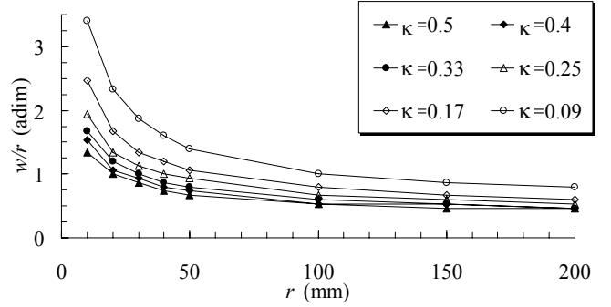
Fig. 15: Ratio between sector width and aperture radius that provides 95% of the maximum critical gradient versus aperture radius for a [0^\circ\text{-}24^\circ, 30^\circ\text{-}36^\circ] sector coil.
