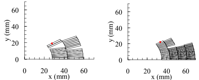
Fig. 8: Coil layouts (one eight shown in the plot) of the LHC MQ (left) and MQY (right).
