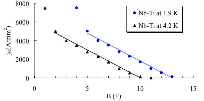
Fig. 1: Critical surface for Nb-Ti at 1.9 K and at 4.2 K, and linear fit given in Eq. (1).
