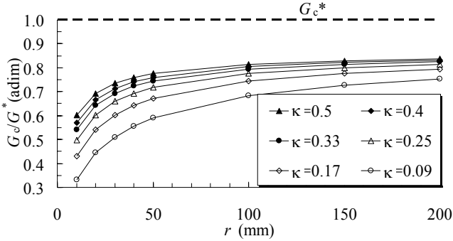
Fig. 14: Ratio between maximum critical gradient and G_c^* given in Eq. (13) versus aperture radius for a [0^\circ\text{-}24^\circ, 30^\circ\text{-}36^\circ] sector coil.
