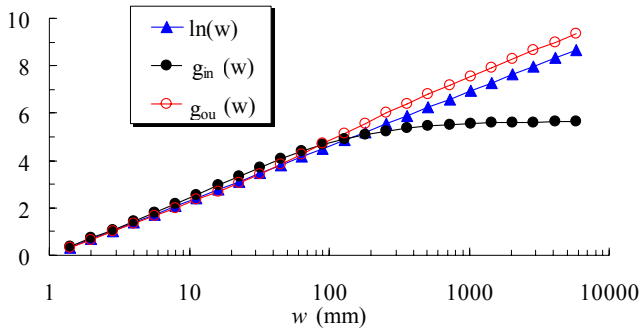
Fig. 29: Functions defined in (B.5), (B.8) and (B.9) versus cable width w for an aperture radius of 30 mm.
