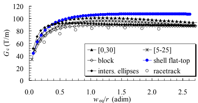
Fig. 23: Numerical evaluation of the critical gradient versus equivalent sector width (41) in six coil layouts with an aperture radius of 100 mm ( \kappa=0.28 ).
