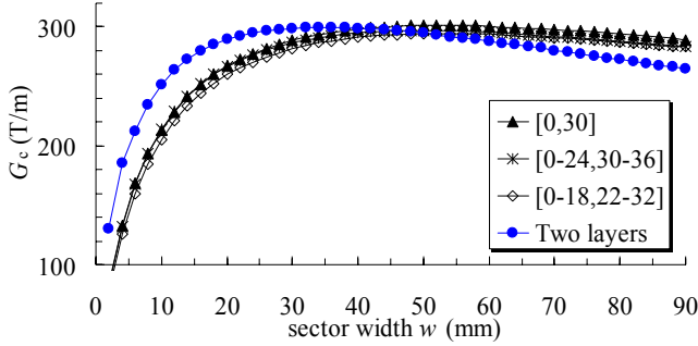
Fig. 11: Numerical evaluation of the critical gradient versus sector width for different sector layouts.
