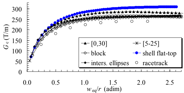
Fig. 22: Numerical evaluation of the critical gradient versus equivalent sector width (41) in six coil layouts with an aperture radius of 30 mm ( \kappa=0.28 ).
