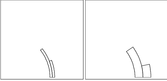
Fig. 9: Two shell layouts solutions \alpha_1=37^\circ, \alpha_2=20^\circ for w/r=0.05 (left) and \alpha_1=35^\circ, \alpha_2=12.5^\circ for w/r=0.16 (right) that set b_6 and b_{10}=0 .
