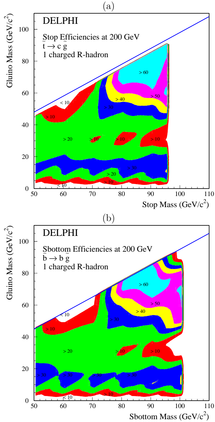
Figure 12: Signal detection efficiencies (%) at \sqrt{s} = 200 GeV for the q\bar{q}R^\pm R^0 analysis, (a) stop, (b) sbottom.
