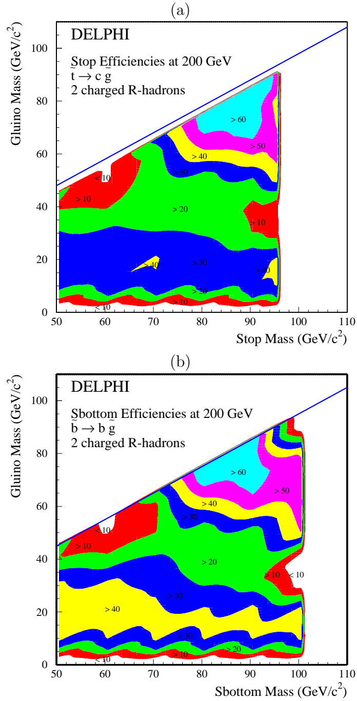
Figure 10: Signal detection efficiencies (%) at \sqrt{s} = 200 GeV for the q\bar{q}R^\pm R^\pm analysis, (a) stop, (b) sbottom.
