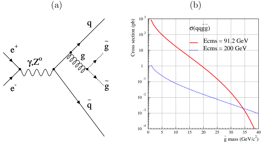
Figure 1: (a) Gluon splitting into a pair of gluinos. (b) Comparison of the cross-section (pb) of this process at centre-of-mass energies of 91.2 GeV (LEP1) and of 200 GeV (LEP2).
