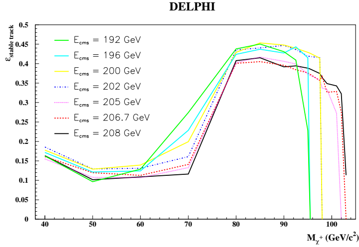
Figure 32: Efficiency for selecting a single almost stable chargino, as function of its mass, at the reference centre-of-mass energies collected by DELPHI in the years 1999 and 2000.
