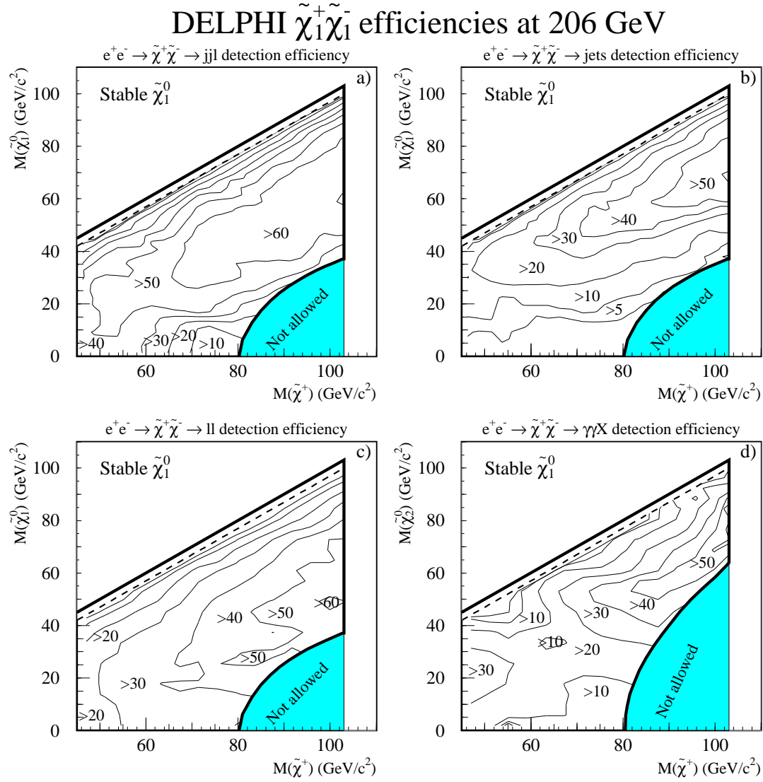
Figure 26: Chargino pair production detection efficiencies (%) for the four decay channels a) jj\ell , b) jets , c) \ell\ell and d) rad , at 206 GeV in the (M_{\tilde{\chi}^\pm}, M_{\tilde{\chi}^0}) plane. TPC sector 6 on and a stable \tilde{\chi}_1^0 are assumed. The shaded areas are disallowed in the MSSM scheme.
