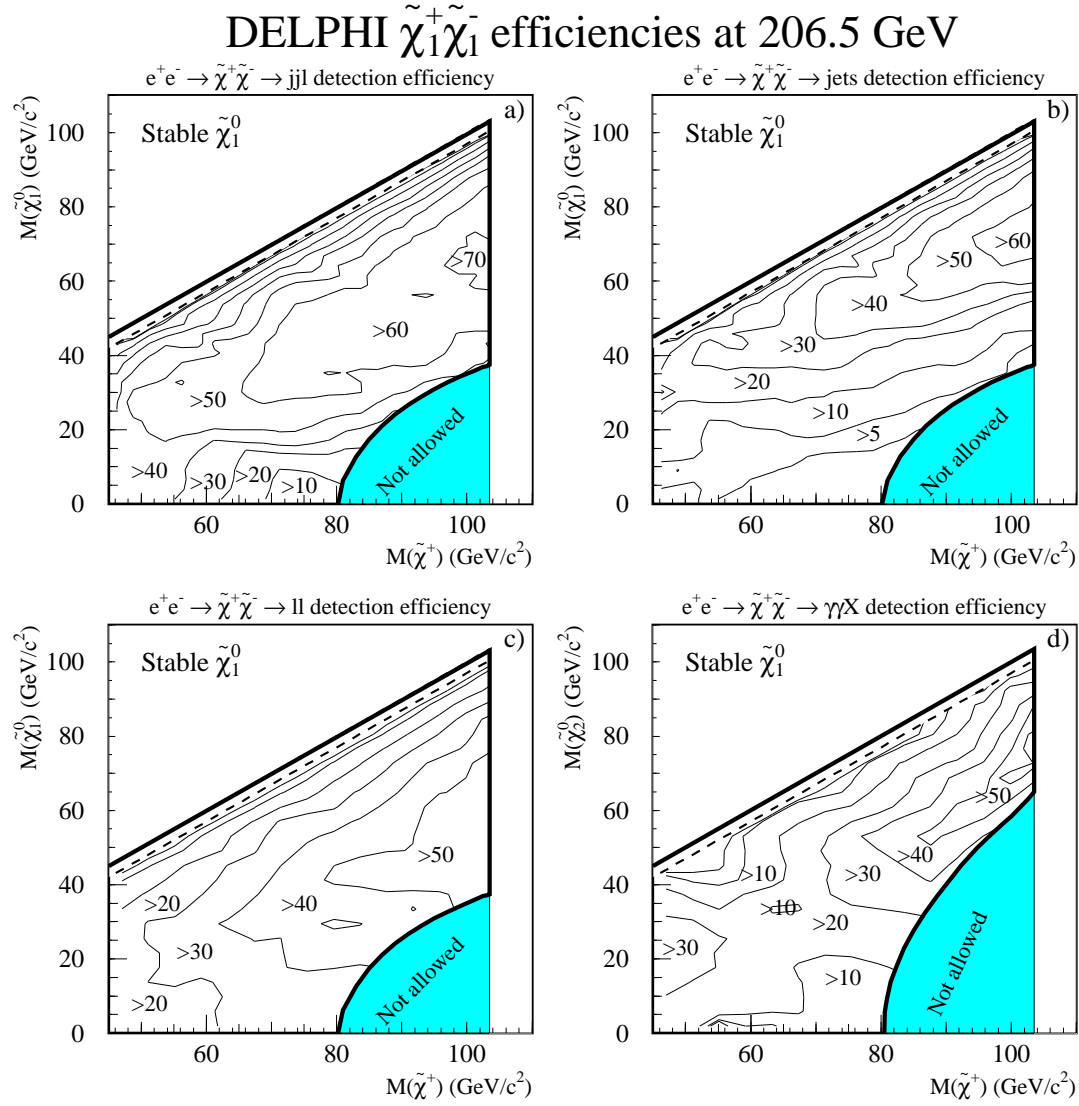
Figure 27: Chargino pair production detection efficiencies (%) for the four decay channels a) jjl , b) jets , c) ll and d) rad , at 206.5 GeV in the (M_{\tilde{\chi}^\pm}, M_{\tilde{\chi}^0}) plane. TPC sector 6 off and a stable \tilde{\chi}_1^0 are assumed. The shaded areas are disallowed in the MSSM scheme.
