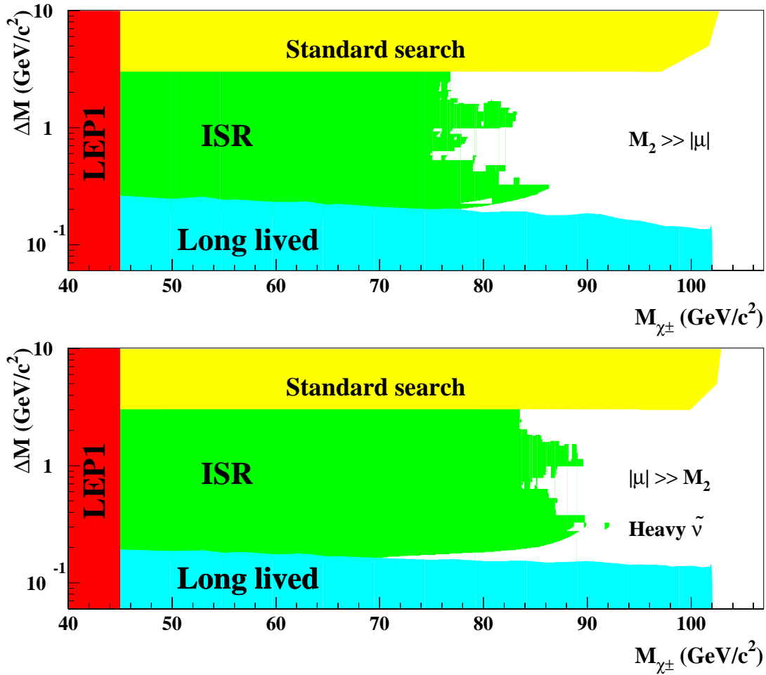
Figure 36: Regions in the plane (M_{\tilde{\chi}_1^+}, \Delta M) excluded by DELPHI at the 95% CL using: the search for high \Delta M charginos; the search for soft particles accompanied by ISR; and the search for long-lived charginos. The two scenarios are (a) the one in which the lightest chargino is a higgsino and (b) the one in which the lightest chargino is a gaugino. For the second scenario, the limits are valid in the heavy sfermion approximation, while for the higgsino scenario it is sufficient that M_{\tilde{f}} > M_{\tilde{\chi}_1^+} .
