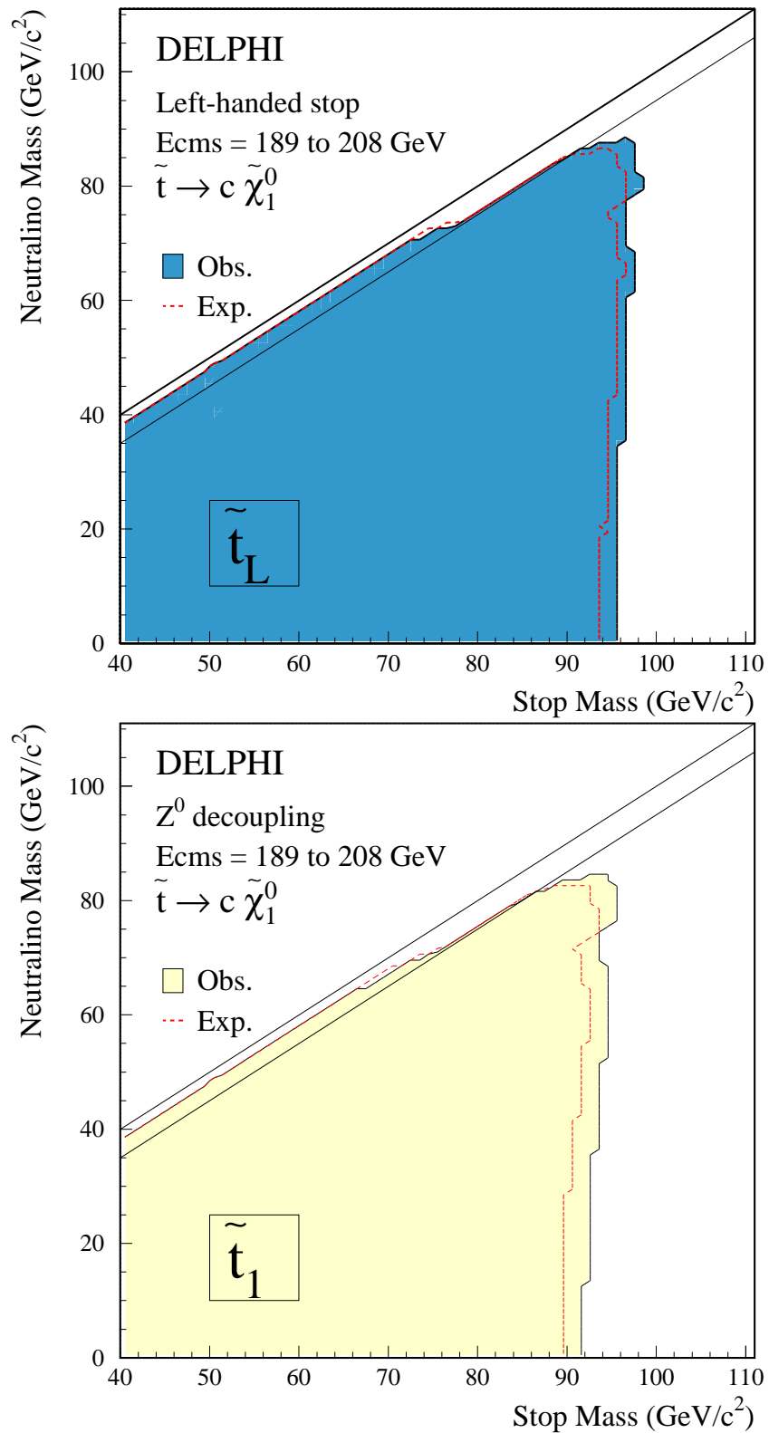
Figure 23: Excluded regions at 95% confidence level for the stop search in the plane (M_{\tilde{t}_1}, M_{\tilde{\chi}_1^0}) for purely left handed stops (top) and for the states at the Z decoupling (bottom). The shaded areas show the observed excluded regions and the lines correspond to the expected exclusions (for a discussion on the low stop mass region see section 6.3).
