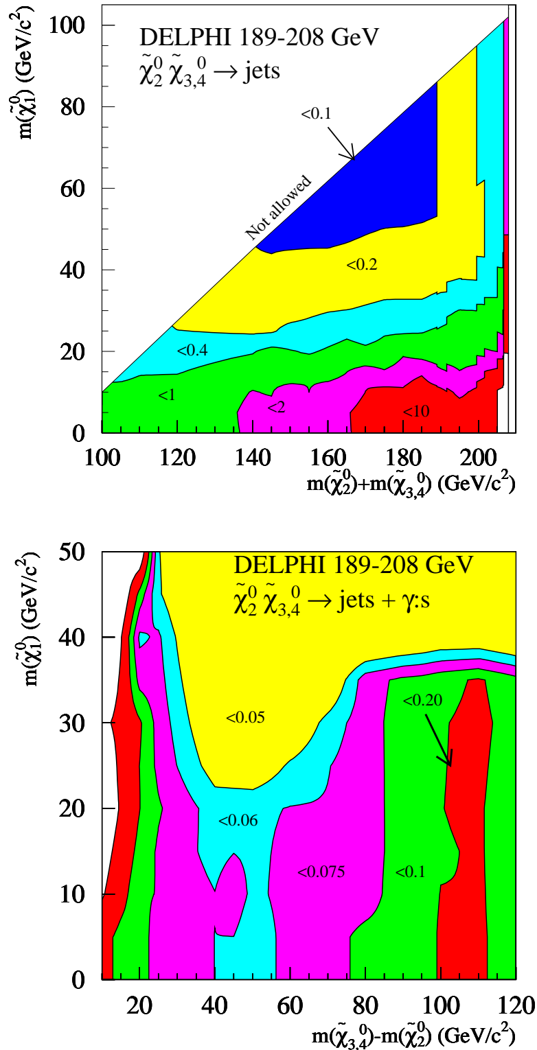
Figure 38: Upper limits on the cross-sections at the 95% confidence level for \tilde{\chi}_2^0 \tilde{\chi}_i^0 production with \tilde{\chi}_i^0 \rightarrow \tilde{\chi}_1^0 q \bar{q} ( i=3,4 ) including data up to \sqrt{s} = 208 GeV. The different shadings correspond to regions where the cross-section limit in picobarns is below the indicated number. The \tilde{\chi}_2^0 was assumed to decay 100% into \tilde{\chi}_1^0 q \bar{q} in a), and into \tilde{\chi}_1^0 \gamma in b). The limits in a) are based on the acoplanar jets and multijets selections, while those in b) derive from the search for multijets with photons.
