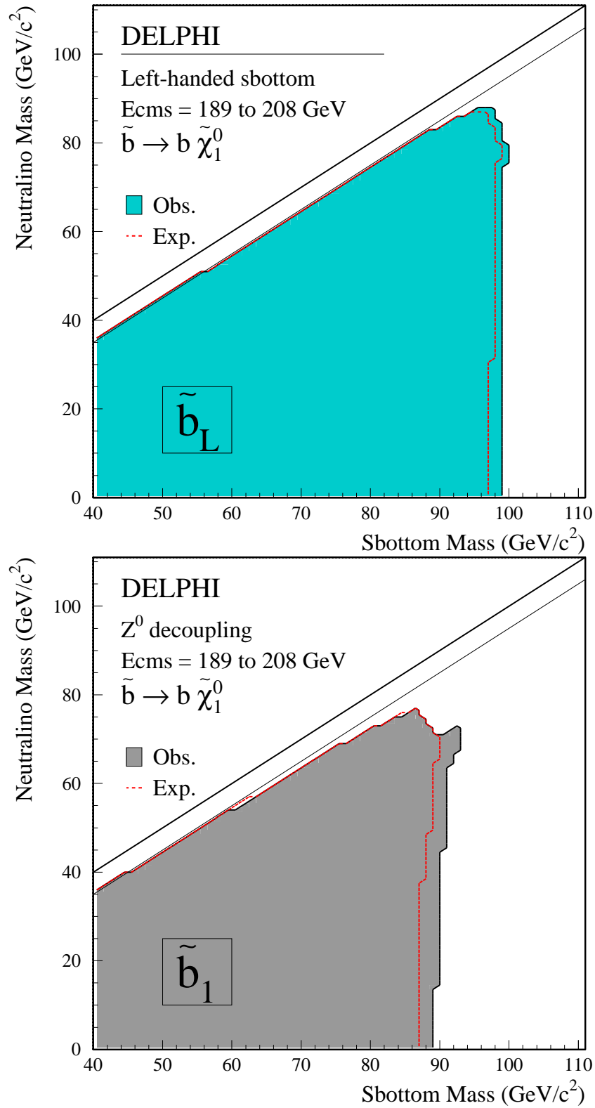
Figure 24: Excluded regions at 95% confidence level for the sbottom search in the plane (M_{\tilde{b}_1}, M_{\tilde{\chi}_1^0}) for purely left handed sbottoms (top) and for the states at the Z decoupling (bottom). The shaded areas show the observed excluded regions and the lines correspond to the expected exclusions (for a discussion on the low sbottom mass region see section 6.3).
