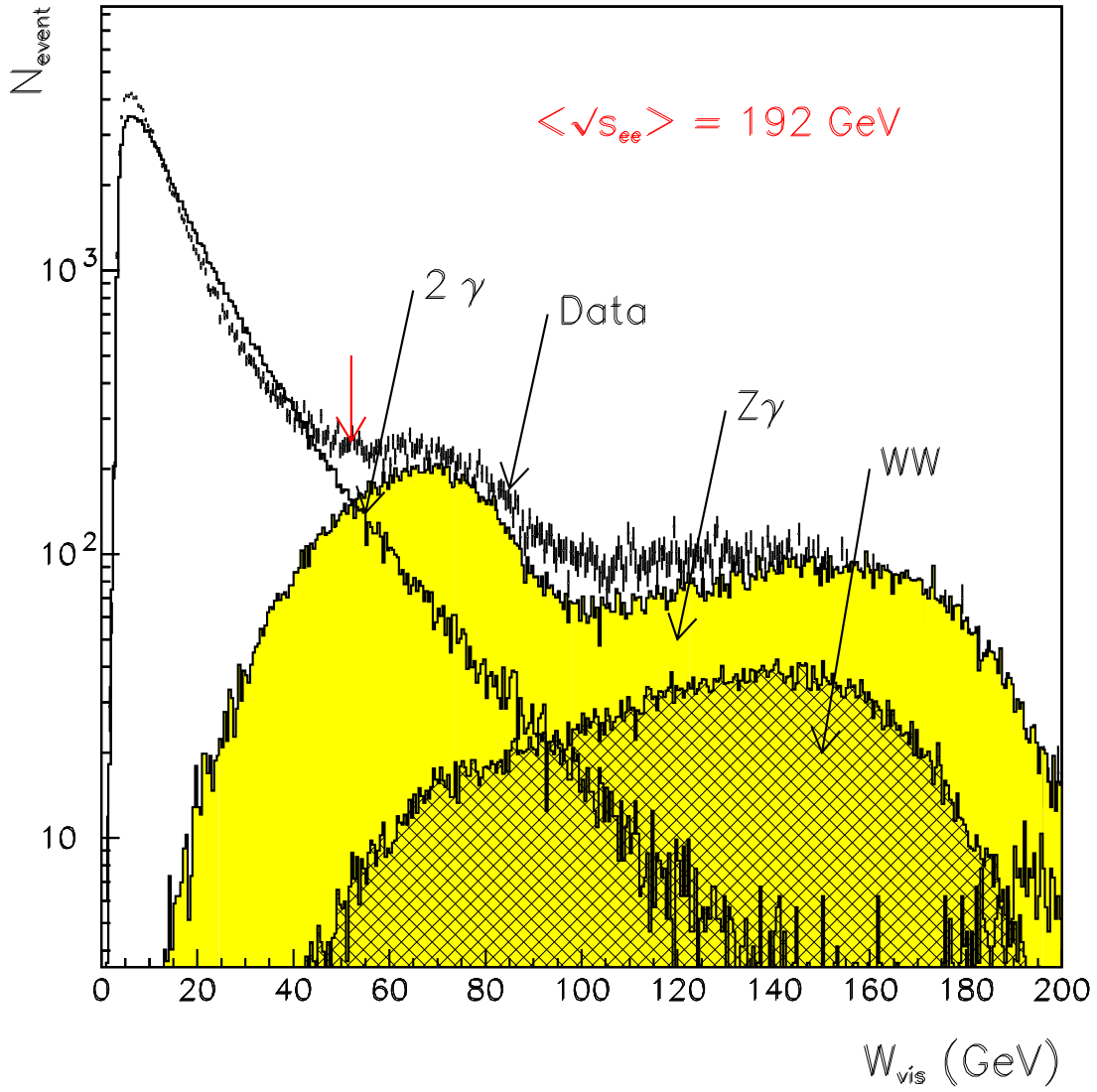
Figure 1: W_{vis} distributions for the data at \langle \sqrt{s_{ee}} \rangle = 192 \text{ GeV} and for the simulated \gamma\gamma \rightarrow \text{hadrons} , e^+e^- \rightarrow Z^0\gamma and e^+e^- \rightarrow W^+W^- events at \sqrt{s_{ee}} = 200 \text{ GeV}
