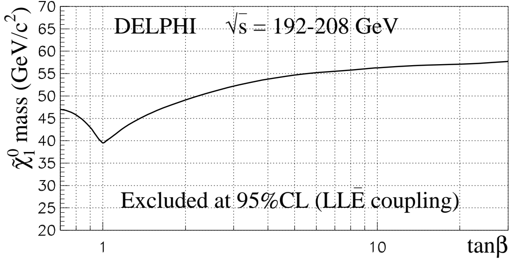
Figure 8: \text{LL}\bar{\text{E}} : excluded lightest neutralino mass as a function of \tan\beta at 95% CL. This limit is independent of the choice of the generation indices i, j, k of the \lambda_{ijk} coupling and is for values of m_0 between 90 and 500 \text{GeV}/c^2 .
