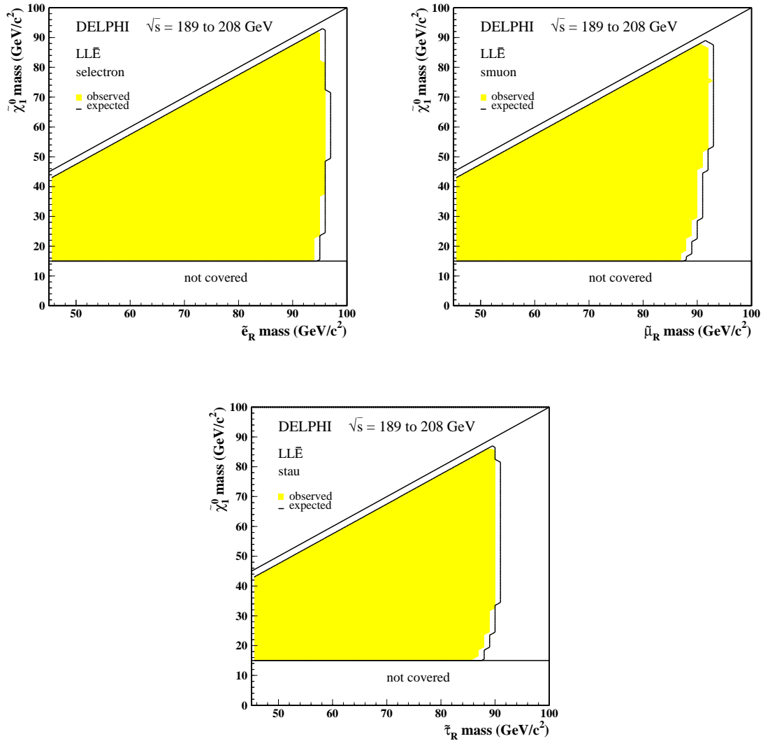
Figure 12: LL \bar{E} : excluded regions at 95% CL in the m_{\tilde{\chi}^0} versus m_{\tilde{\ell}_R} planes for \tilde{\ell}_R pair-production, with \text{BR}(\tilde{\ell}_R \rightarrow \tilde{\chi}_1^0 \ell) = 100\% , and neutralino decay into leptons. The plots show the exclusion (filled area) for selectron, smuon and stau. The black contour is the corresponding expected exclusion at 95% CL.
