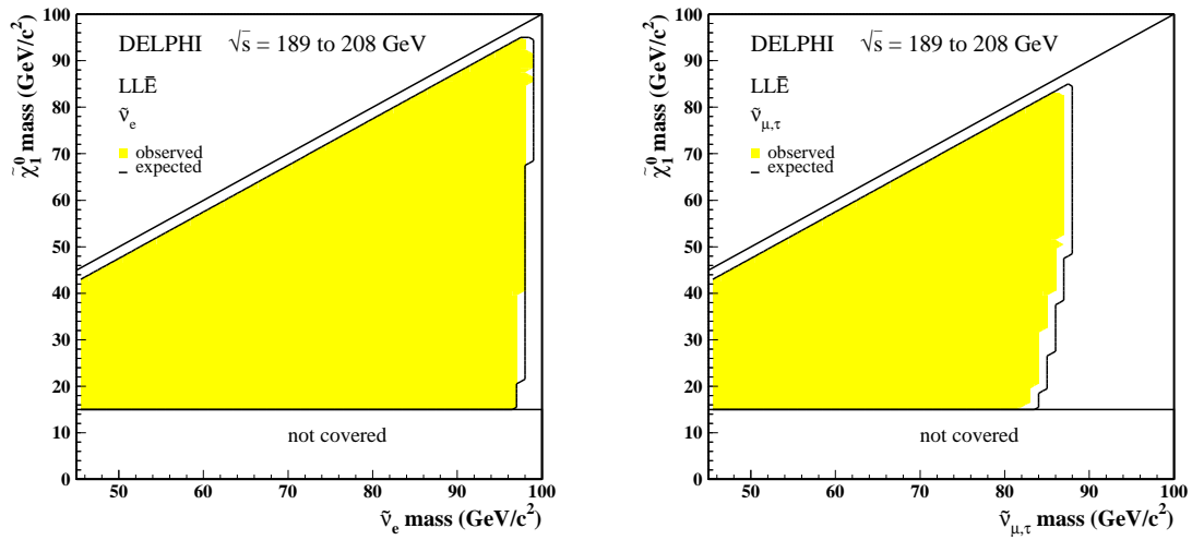
Figure 13: LL \bar{L} : excluded regions at 95% CL in the m_{\tilde{\chi}^0_1} versus m_{\tilde{\nu}} planes for \tilde{\nu}_e (left) and \tilde{\nu}_\mu, \tilde{\nu}_\tau (right) pair-production, with \text{BR}(\tilde{\nu} \rightarrow \tilde{\chi}^0_1 \nu) = 100\% , and neutralino decay into leptons. The black contour is the corresponding expected exclusion at 95% CL.
