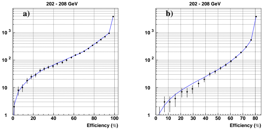
Figure 9: \bar{\text{U}}\bar{\text{D}}\bar{\text{D}} : number of expected events (continuous line) and data events (black dots) versus average signal efficiency for the high neutralino mass search N3 (plot a) and for the large \Delta M chargino search C2 (plot b) for centre-of-mass energies between 202 and 208 GeV.
