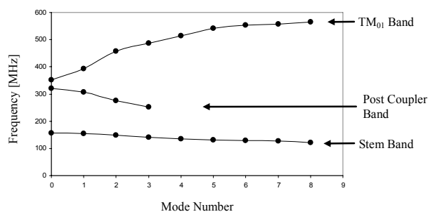
Figure 2: Computed mode frequencies in 1/3 of Tank 1.
