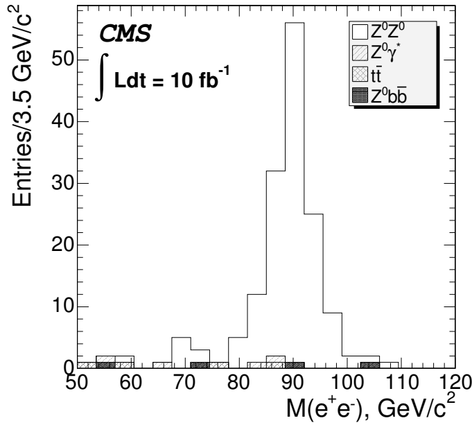
Figure 2: Distribution of the mass of the Z^0 candidates, two entries per event, retained by the Z^0 Z^0 selection, for an integrated luminosity of 10\text{fb}^{-1} .
