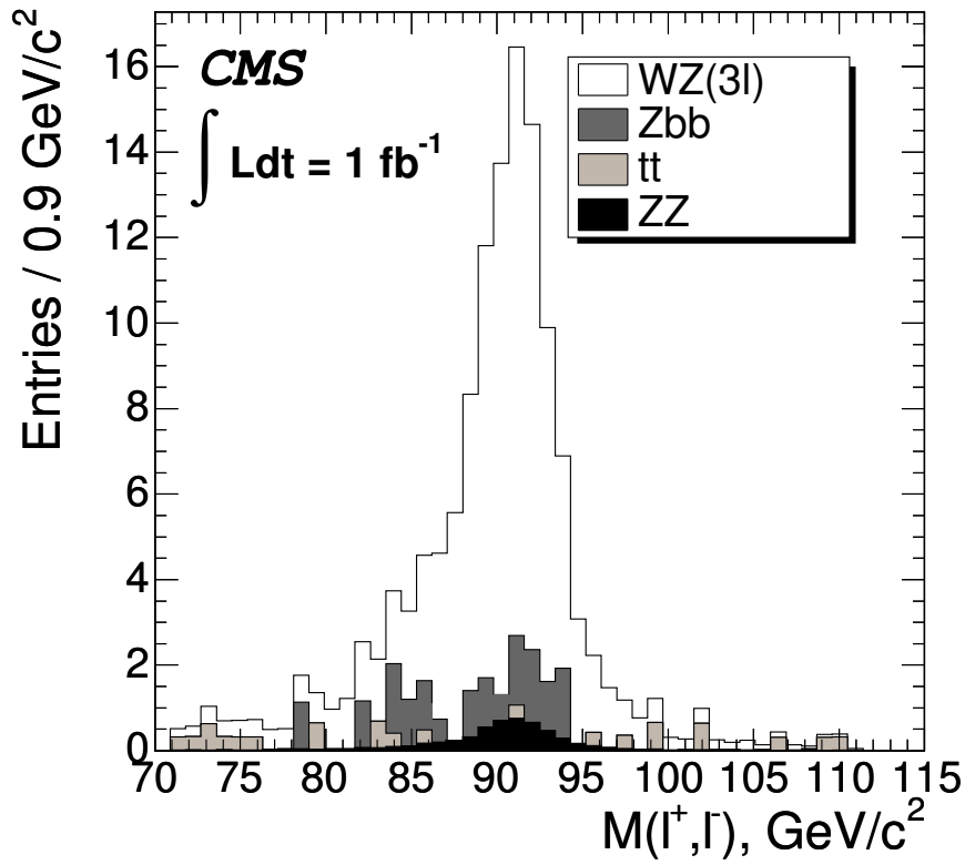
Figure 1: Distribution of the mass of the Z^0 candidates for events retained by the W^\pm Z^0 selection, for an integrated luminosity of 1\text{fb}^{-1} .
