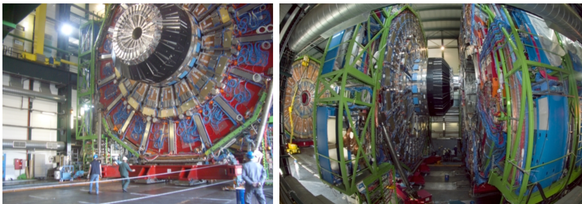
Figure 4. CMS assembly process: YE1 (left) equipped with the muons chambers and calorimeters sliding on the floor towards YB3 (right).
