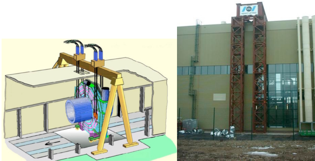
Figure 3. Heavy lifting principle (left). Elements of the crane (right) as installed on P5
