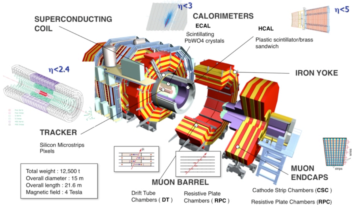
Figure 1. Overview of the CMS detector
