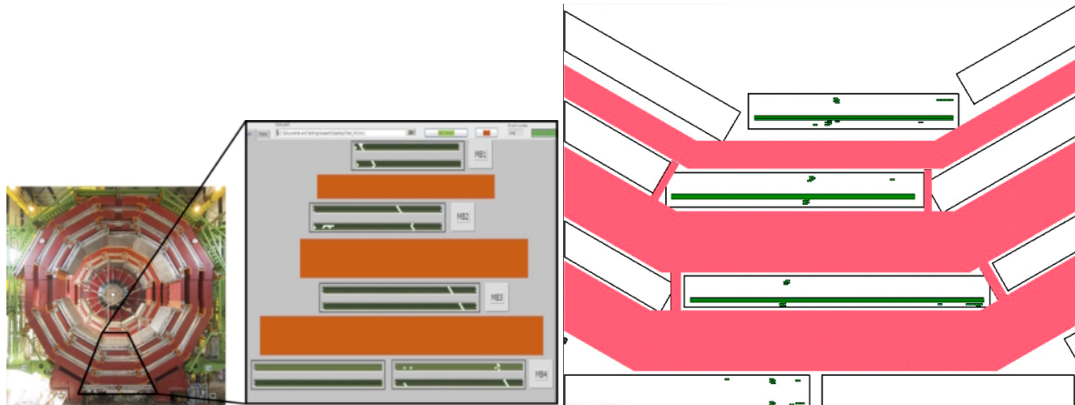
Figure 7. Muon data recorded in CMS DT chambers without magnetic field (left) and with field on (right)
