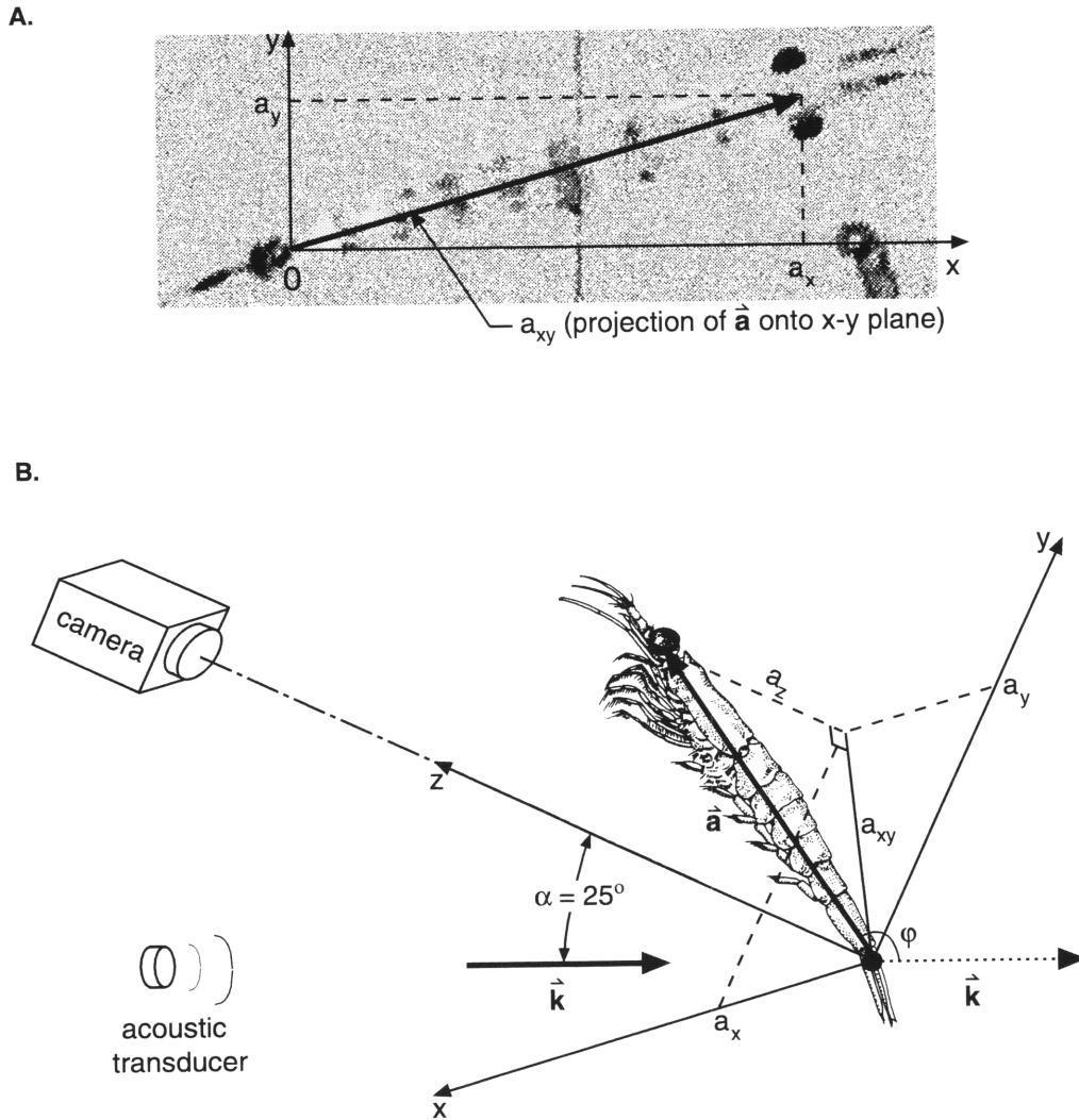
Figure 5-9 Geometry for determination of angle of orientation \phi from the video images. A. Image gives the projection of the animal vector \vec{a} onto the x-y plane of a 3-D coordinate system with origin situated at the base of the krill's telson. a_x and a_y computed directly from measurements made of the image; B. a_z determined from geometry shown; \phi computed using (EQ 5.2); incident acoustic wave vector \vec{k} is in the y-z plane, at an angle of \alpha = 25^\circ relative to the camera line of sight.
