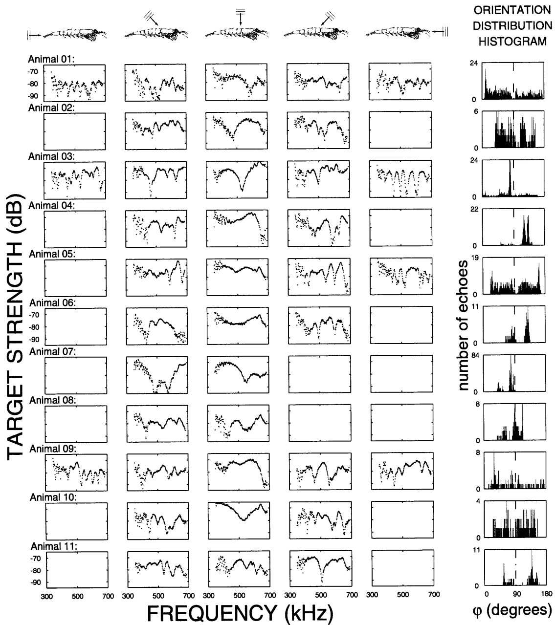
Figure 5-10 Examples of echo spectra received from 11 krill (Animals 01 through 11, rows) at 5 angles of orientation, with acoustic wave incident at \phi \cong 0^\circ, 45^\circ, 90^\circ, 135^\circ, 180^\circ (\pm 15^\circ) (first 5 columns); empty plots indicate that the animal did not assume that orientation during the experiment. Histogram of orientation distribution for each animal during insonification shown at right.
