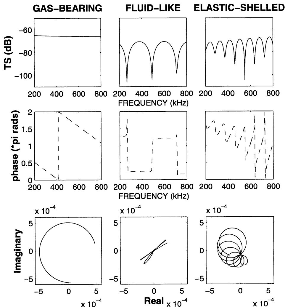
Figure 2-6 Characteristics of the theoretical-model-generated clean signals. Top row is |S(\omega)| , the magnitude of the Fourier transform of s(t) , plotted as target strength (TS) in dB. Second row is the phase of S(\omega) , computed as \tan^{-1}(\text{Re}[S(\omega)]/\text{Im}[S(\omega)]) . Bottom row is the phasor diagram, showing plot of \text{Im}[S(\omega)] vs. \text{Re}[S(\omega)] over the frequency band 200 kHz - 800 kHz. Theoretical models plotted above are explicitly described in (EQ 3.1) with b_j = 0 ( GB ), (EQ 3.2) with N = 2 ( FL ) and (EQ 3.5) with the series truncated to include only the first partial circumnavigation ( ES ).
