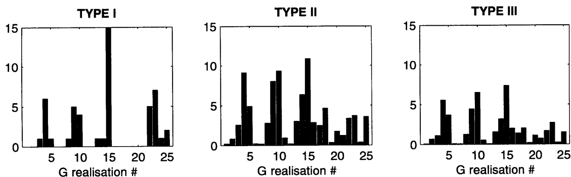
Figure 4-8 Class-support TYPE I , TYPE II and TYPE III PMFs f^{(s)} , computed using (EQ 4.12), for the simplified model space G (a first-order representation of the model space for the GB scattering class). For TYPE II and TYPE III f, t_f = 0.5 \max(C_{f_{ij}}^{(p)}) . The validation set V^{(3)} contains 50 observed echo spectra from a single siphonophore ( Agalma okeni ).
