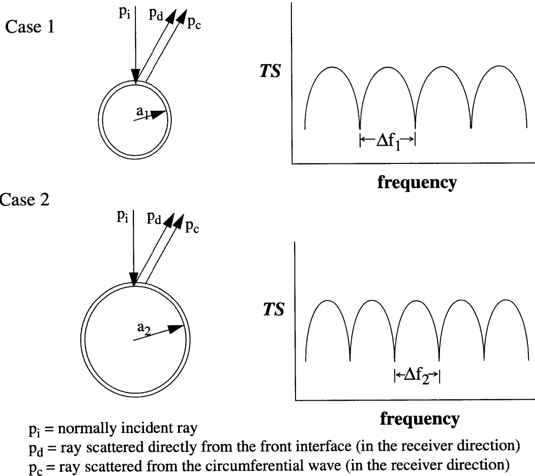
Figure 5-5 Schematic of an elastic-shelled animal insonified at high frequency ( \lambda \gg a ), comparing spectra scattered from a small animal of radius a_1 (Case 1) vs. a larger animal of radius a_2 > a_1 (Case 2).
