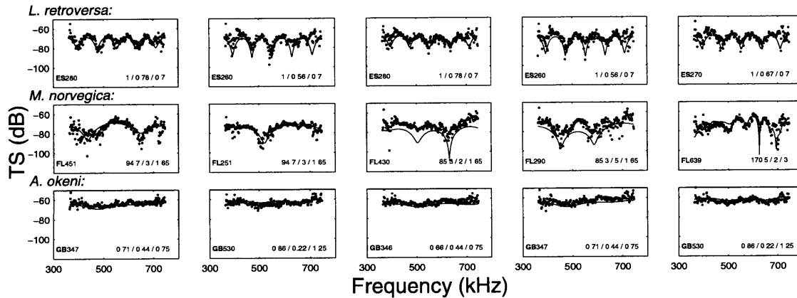
Figure 4-12 Selected examples of PSC-inverted best match echo classifications for five observations each of a pteropod L. retroversa ( \bar{a} \cong 0.75 mm, top), a euphausiid M. norvegica ( a \cong 1.5 - 2 mm, middle), and a siphonophore A. okeni ( a \cong 0.6 - 1 mm, bottom), from the high-quality subset of 1993 data. Observations (points) plotted together with best match model realisations (solid line); best match scattering class and model realisation number shown at bottom left, parameter inversions given at bottom right ( ES : F_{spec}/F_l/\bar{a} ; FL : \beta_{tilt}/shape\#/a ; GB : F_{tiss}/\epsilon_f/a ; \bar{a} and a in mm, \beta_{tilt} in degrees). PSC implemented including both ambiguity and validity weightings ( \bar{W}_A , \bar{W}_V ). Validation set V included half of the 1550 1993 observations. Classification threshold t was adjusted to include all CMV within the 3 dB-down range: t = 0.5\max(C_v^{(p)}) .
