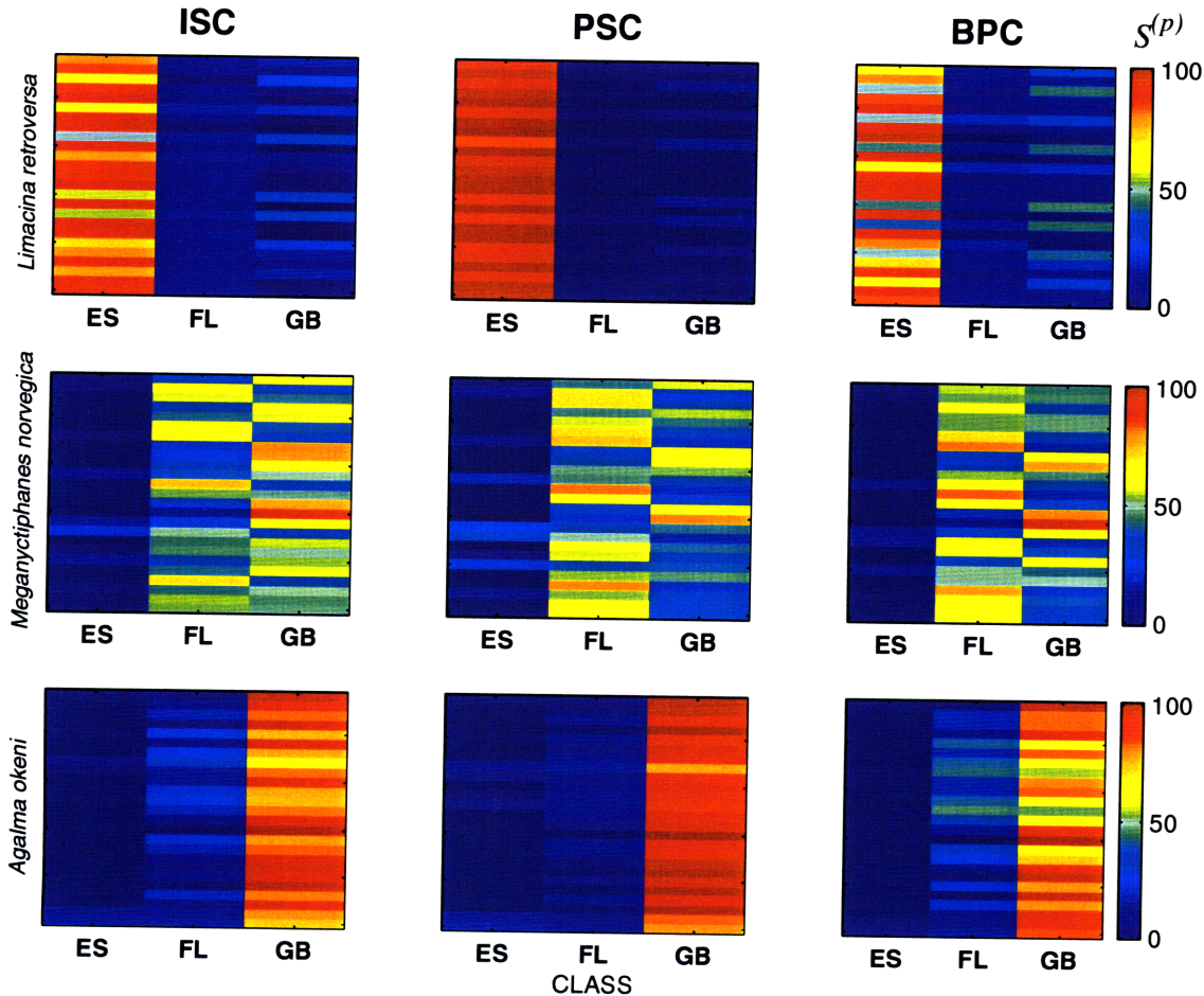
Figure 4-10 Classification scores for the Integrated Score Classifier (ISC; left, \mathcal{S}_{ISC}^{(p)} \times 100 ), Pairwise Score Classifier (PSC; center, \mathcal{S}_{PSC}^{(p,p)} ) and Bayesian Probability Classifier (BPC; right, \mathcal{S}_{BPC}^{(p)} ) for a selected subset of the highest quality data (25 acoustic returns each (y-axis) from an elastic-shelled pteropod Limacina retroversa , top row, a fluid-like euphausiid Meganyctiphanes norvegica , middle row, and a gas-bearing siphonophore Agalma okeni , bottom row). Scores \mathcal{S}^{(p)} colour-coded according to the legend (right). ISC and PSC implemented including both ambiguity and validity weightings ( \tilde{W}_A , \tilde{W}_V ); BPC implemented using a class-support TYPE II \mathbf{f}^{(p)} with t_f = 0.5 \max(\mathbf{C}_{f_{ij}}^{(p)}) . Validation set \mathbf{V} included half of the 1550 observations from the 1993 dataset. Classification threshold t was adjusted to include all CMV within the 3 dB-down range: t = 0.5 \max(\mathbf{C}_{f_{ij}}^{(p)}) .
