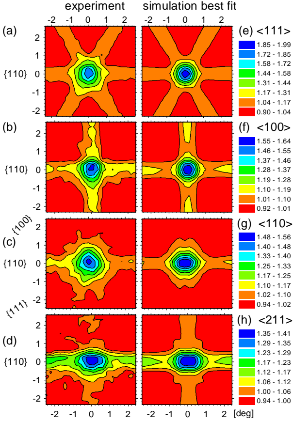
FIG. 3. (a)-(d): Experimental emission channeling patterns from sample #8 following annealing at 800°C. (e)-(h): Best fit results, corresponding to (e) 29% (S+T), 61% near-(S+T), and 10% (R), (f) 43% (S+T), 91% near-(S+T), and -34% (R), (g) 50% S, 0% near-S, 35% near-T, and 15% (R), (h) 30% S, 10% near-S, and 34% near-T, and 26% (R).
