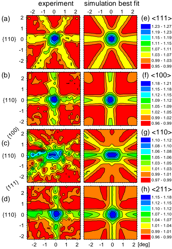
FIG. 1. (a)-(d): Normalized \beta^- emission yield from sample #8 in the vicinity of \langle 111 \rangle , \langle 100 \rangle , \langle 110 \rangle , and \langle 211 \rangle directions following annealing at 300^\circ\text{C} . (e)-(h): Best fit results, corresponding to (e) 5% (S+T), 54% near-(S+T), and 41% R, (f) 12% (S+T), 61% near-(S+T), and 27% R, (g) 3% S, 41% near-S, 22% near-T, and 34% R, (h) 0% S, 39% near-S, 21% near-T, and 40% R.
