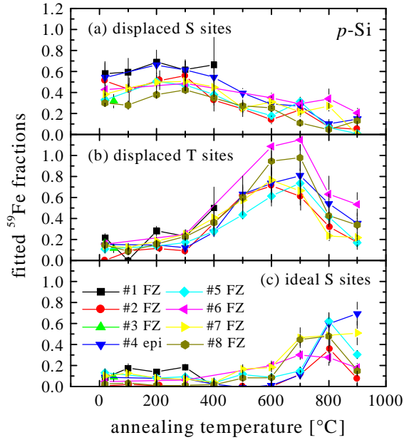
FIG. 4. Fractions of ^{59}\text{Fe} on the three different lattice sites for the p -type samples #1 to 8, derived from fits to the experimental patterns assuming an as-implanted depth profile of ^{59}\text{Fe} . Sample #3 was only annealed up to 50°C and sample #1 only up to 400°C.
