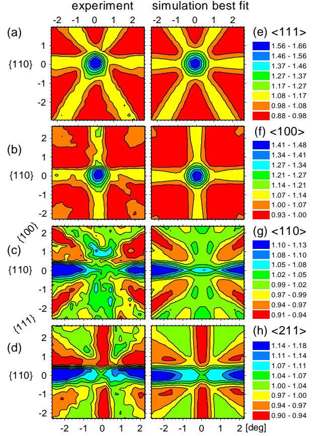
FIG. 2. (a)-(d): Experimental emission channeling patterns from sample #8 following annealing at 600^\circ\text{C} . (e)-(h): Best fit results, corresponding to (e) 30% (S+T), 113% near-(S+T), and -43\% (R), (f) 30% (S+T), 104% near-(S+T), and -34\% (R), (g) 11% S, 14% near-S, 75% near-T, and 0% (R), (h) 3% S, 34% near-S, 99% near-T, and -36\% (R).
