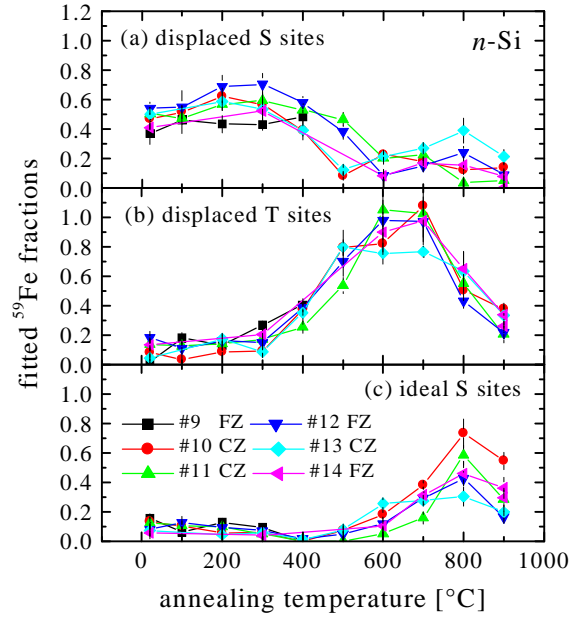
FIG. 5. Fractions of ^{59}\text{Fe} on the three different lattice sites for the n -type samples #9 to 14, derived from fits to the experimental patterns assuming an as-implanted depth profile of ^{59}\text{Fe} . Sample #9 was only annealed up to 400°C.
