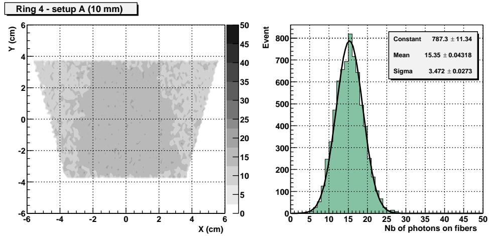
Figure 12: Number of scintillation photons collected by fibers as a function of the impact point of the particle on the element of the ring 4. Results are obtained from simulation of the setup A configuration with 8 fibers.
