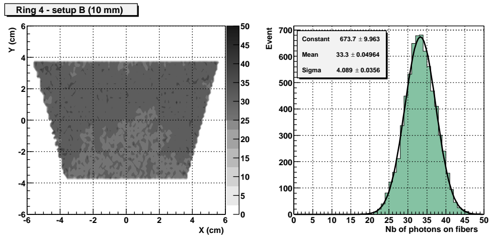
Figure 13: Number of scintillation photons collected by fibers as a function of the impact point of the particle on the element of the ring 4. Results are obtained from simulation of the setup B configuration with 16 fibers.
