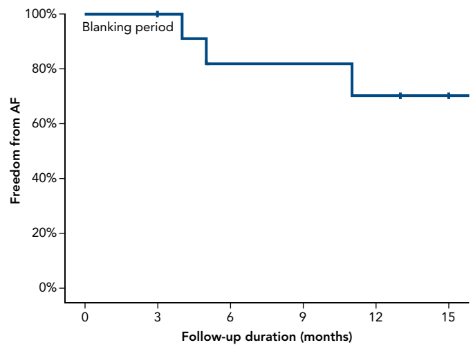
Figure 1: Freedom From AF During Follow-up Following Cryoballoon Ablation
