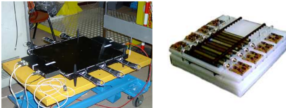
Fig. 16. Left: the shower tail catcher scintillator, S4, showing the 6 PMTs used for read-out. The scintillator has dimensions (48 \times 48) cm 2 . Right: The neutron detector partially equipped with 3 He proportional counters. The neutron detector covers an area of (60 \times 55) cm 2 .
