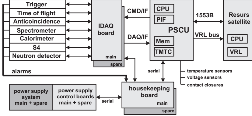
Fig. 17. Scheme of the PAMELA data acquisition system. The interfaces (IF) between the IDAQ and the PSCU handle the data acquisition and transfer the commands (CMD) to the IDAQ. The communication between PAMELA and the spacecraft is handled by the 1553B bus and by the link to the VRL module for data download to the Resurs memory. Adapted from [52].
