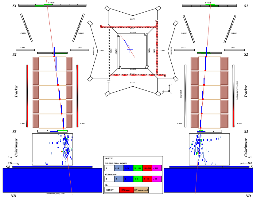
Fig. 27. The event display of a \sim 13 GV interacting helium nucleus from flight data. On the left (right) the x, bending (y, non-bending view) of PAMELA are indicated. A plan view of PAMELA is shown in the centre. Note the increased energy deposit in the silicon tracker planes (denoted by the vertical bars) compared to figure 26. The activity in the anticounter system is probably due to secondary particles backscattered from the calorimeter.
