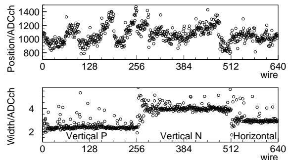
Figure 5. Pedestal positions and widths
