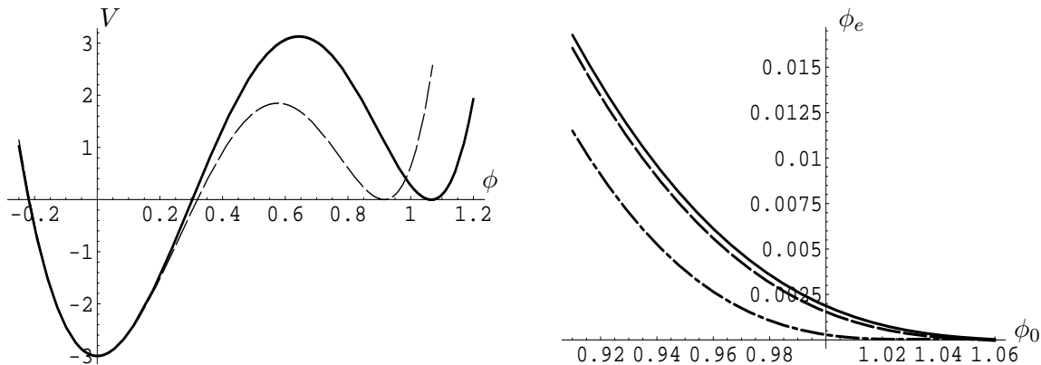
Figure 7: The left panel shows a potential (full line) that is on the verge of violating the PET for asymptotically flat solutions. Also shown is a small deformation of this potential (dashed line) that does not satisfy the PET. The right panel shows how \phi_e , the value of \phi at the horizon of regular spherical asymptotically flat hairy black holes, changes, for three different values of R_e , when one decreases A from A \approx 65 toward its critical value A_c = 57.6 , while keeping the local minimum at zero. This corresponds to a deformation where the potential changes from the dashed line in the left panel, for which \phi_0 = .92 , to the one given by the full line where \phi_0 = 1.06 . The full line in the right panel shows \phi_e as a function of \phi_0 for R_e = 5 , the dashed line corresponds to R_e = 2 black holes and the dot-dashed line to R_e = 1 . One sees that for all radii R_e , \phi_e \rightarrow 0 when A \rightarrow A_c . There are no regular asymptotically flat hairy black holes for A < A_c .
