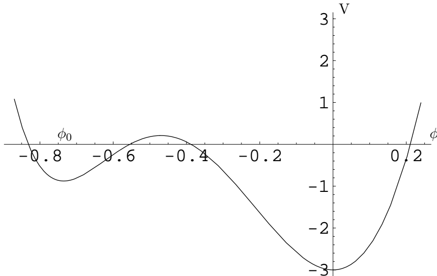
Figure 1: A potential V(\phi) that is on the verge of violating the Positive Energy Theorem for solutions that asymptotically approach the local AdS minimum at \phi_0 .
