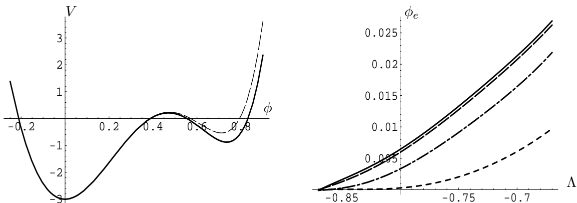
Figure 9: The left panel shows a potential (full line) that is on the verge of violating the PET for solutions where \phi asymptotically decays to the local AdS minimum at \phi_0 . The potential that is given by the dashed line does not satisfy the PET for these asymptotic conditions. The right panel shows \phi_e as a function of \Lambda = V(\phi_0) , for four different values of R_e , when one decreases \Lambda towards its critical value \Lambda_c = -.88 . The full line in the right panel corresponds to R_e = 10 , the dashed line to R_e = 5 , the dot-dashed line to R_e = 2 and the dotted line to R_e = 1 . One sees that for all radii R_e , \phi_e \rightarrow 0 precisely when \Lambda \rightarrow \Lambda_c . There are no regular spherical hairy black holes where \phi \rightarrow \phi_0 at infinity for \Lambda < \Lambda_c when the false vacuum is stable.
