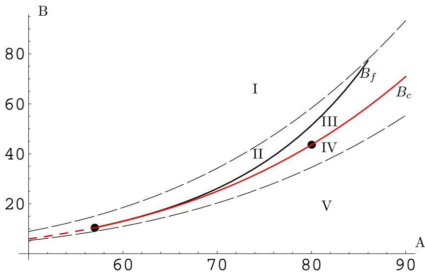
Figure 2: The function B_c(A) represents a set of critical potentials of the form (3.2), with a local AdS minimum at \phi_0 < 0 and a global minimum at \phi = 0 . The function B_f(A) corresponds to potentials with a local minimum at \phi_0 where V(\phi_0) = 0 . The combination (A, B) = (57.6, 10.87) where B_c = B_f yields a critical potential with a local minimum at zero.
