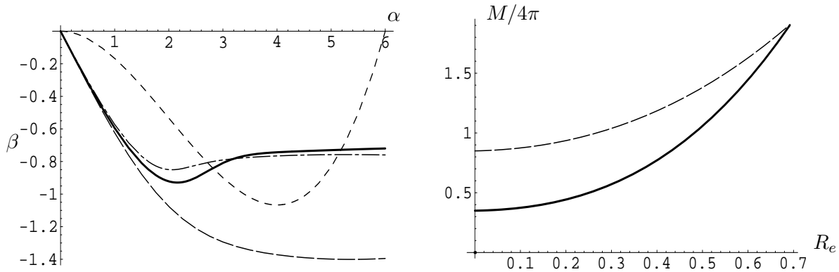
Figure 5: The left panel shows the functions \beta(\alpha) obtained from the solitons and from hairy black holes of two different sizes. The full line shows the soliton curve \beta_s(\alpha) , the dot-dashed line shows the \beta_{R_e}(\alpha) curve for R_e = .2 black holes and the dashed line is the R_e = 1 curve. One sees the boundary condition function \beta_{bc}(\alpha) = -\frac{1}{5}\alpha^2 + \frac{1}{30}\alpha^3 , given by the dotted line, intersects the curves \beta_{R_e}(\alpha) twice for small R_e . The right panel shows the mass of the hairy black holes that obey these boundary conditions. The full line gives the masses of the second (perturbatively stable) branch of solutions, which are associated with the second intersection point of the curves \beta_{R_e}(\alpha) with \beta_{bc}(\alpha) , and hence have more hair.
