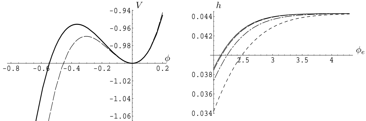
Figure 10: The left panel shows a potential (full line) that is unbounded from below, and on the verge of violating the PET for asymptotically AdS solutions. The right panel shows how \phi_e changes, for four different values of R_e , when one increases the height h of the barrier to its critical value h_c = .044 . The full line in the right panel corresponds to R_e = 10 , the dashed line to R_e = 5 , the dot-dashed line to R_e = 2 and the dotted line to R_e = 1 . One sees that for all radii R_e , \phi_e \rightarrow \infty when the height of the barrier reaches its critical value. For h > h_c there are no regular asymptotically AdS black holes with spherical scalar hair.
