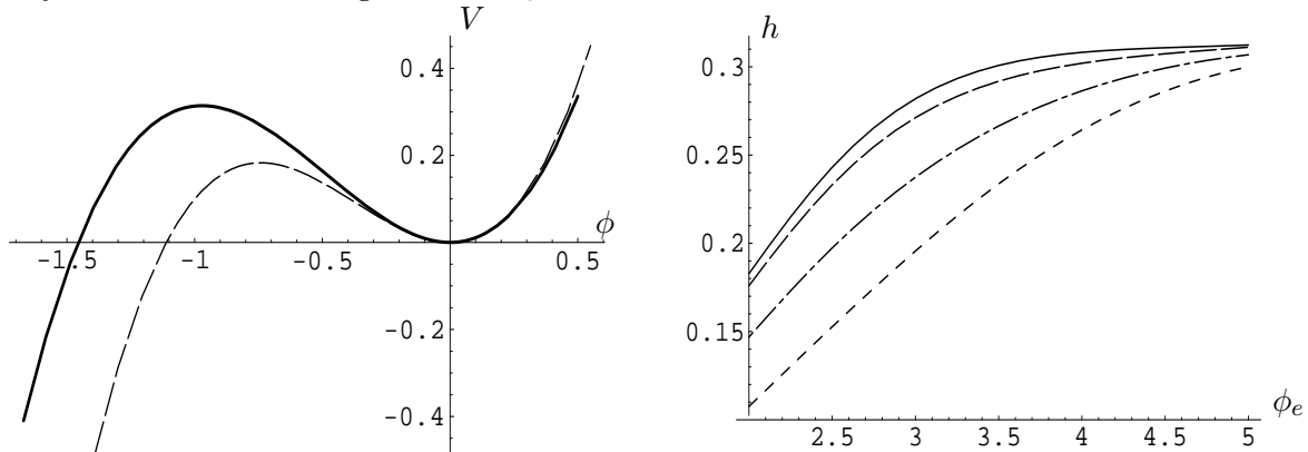
Figure 8: The left panel shows a potential (full line) that is unbounded from below, and on the verge of violating the PET for asymptotically flat solutions. The right panel shows how \phi_e changes, for four different values of R_e , when one increases the height h of the barrier to its critical value h_c = .3 . The full line in the right panel corresponds to R_e = 10 , the dashed line to R_e = 5 , the dot-dashed line to R_e = 2 and the dotted line to R_e = 1 . One sees that for all radii R_e , \phi_e \rightarrow \infty when the height of the barrier reaches its critical value. For h > h_c there are no regular asymptotically flat hairy black holes.
