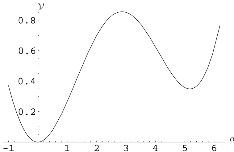
Figure 6: The effective potential \mathcal{V}(\alpha) for the vacuum expectation values \langle \mathcal{O} \rangle in the dual field theory with deformation W = -\frac{1}{15}\alpha^3 + \frac{1}{120}\alpha^4 .
