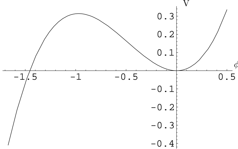
Figure 4: A potential V(\phi) that is on the verge of violating the the Positive Energy Theorem for solutions that asymptotically approach the local minimum at \phi = 0 .
