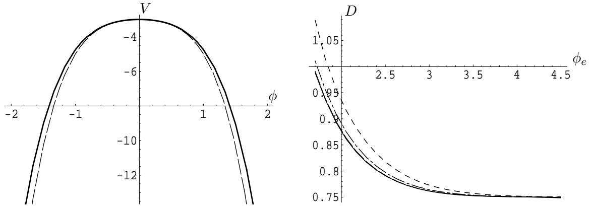
Figure 11: The left panel shows a potential (full line) that is on the verge of violating the PET for solutions where \phi asymptotically decays as \sim 1/r^2 to the local maximum at \phi = 0 . It has m^2 = -2 and a critical negative quartic coupling -D\phi^4 where D_c = 3/4 . The potential given by the dashed line has D > D_c , and hence violates the PET for the same asymptotic conditions. The right panel shows how \phi_e , the value of \phi at the horizon of regular hairy black holes where \phi \sim 1/r^2 at infinity, changes, for four different values of R_e , when one decreases the coupling constant D from D \approx 1 to its critical value D_c . The full line in the right panel corresponds to R_e = 10 , the dashed line to R_e = 5 , the dot-dashed line to R_e = 2 and the dotted line to R_e = 1 . One sees that in all cases, \phi_e \rightarrow \infty when D \rightarrow D_c . For D < D_c the scalar hair of regular asymptotically AdS black holes behaves as \phi \sim 1/r + \mathcal{O}(1/r^2) for all \phi_e .
