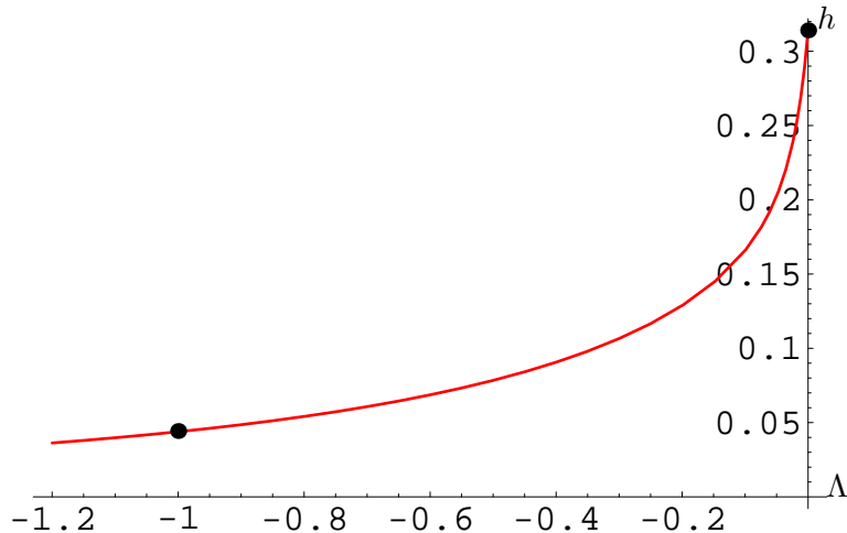
Figure 3: The function h_c(\Lambda) that specifies a set of critical potentials of the form (3.3), which are unbounded from below.
