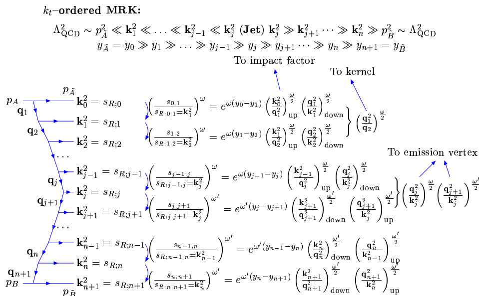
Figure 5: Momenta for 2 \rightarrow 2 + (n - 1) + \text{jet} amplitude in the asymmetric configuration with k_t -ordered MRK.
