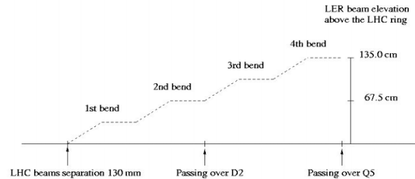
Figure 4: Beam transfer LER-LHC, 4 bends are used to get clear of the LHC magnets.
