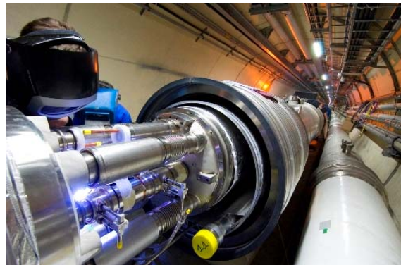
Figure 1: The former LEP tunnel to house the LHC.
