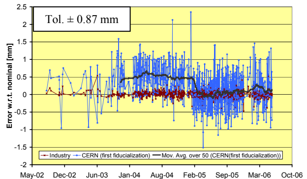
Figure 2: End flanges after fiducialization at CERN.
