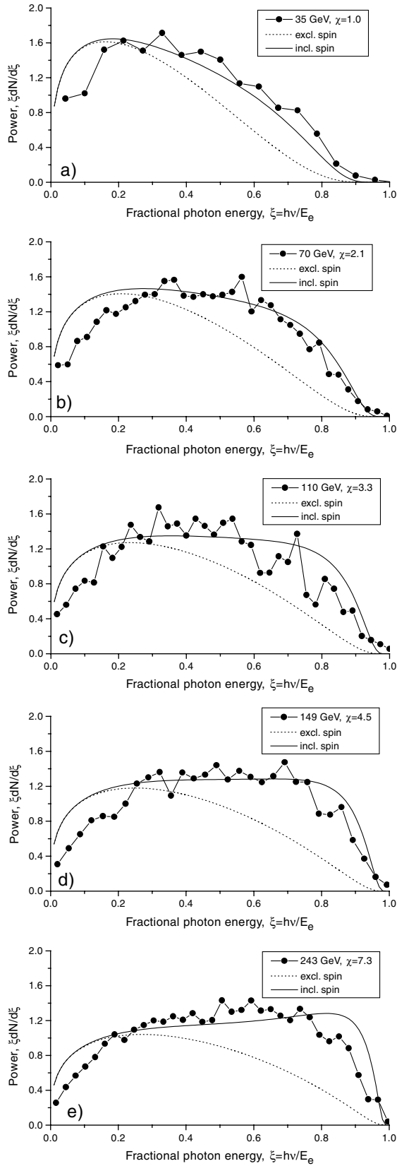
FIG. 1. Power spectrum of radiated photons, \xi dN/d\xi , for electrons aligned 0.3 mrad from the axis in 0.2 mm W \langle 111 \rangle . Filled circles denote the experimental points and the lines (full line = incl. spin; dotted line = excl. spin) the calculated values.
