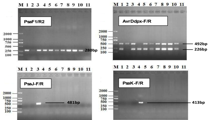
Figure 1 PCR identification of Psa with multiple primers.
