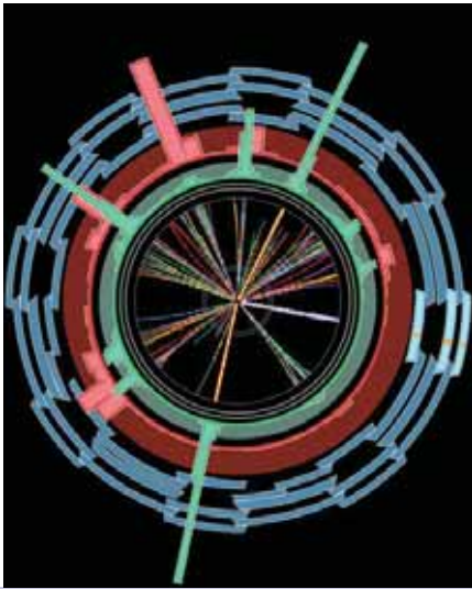
Particle fireworks. Each collision gives rise to a spray of new particles such as these, simulated in the ATLAS detector. This pattern shows what the detector would see if a mini black hole were produced and immediately decayed.
