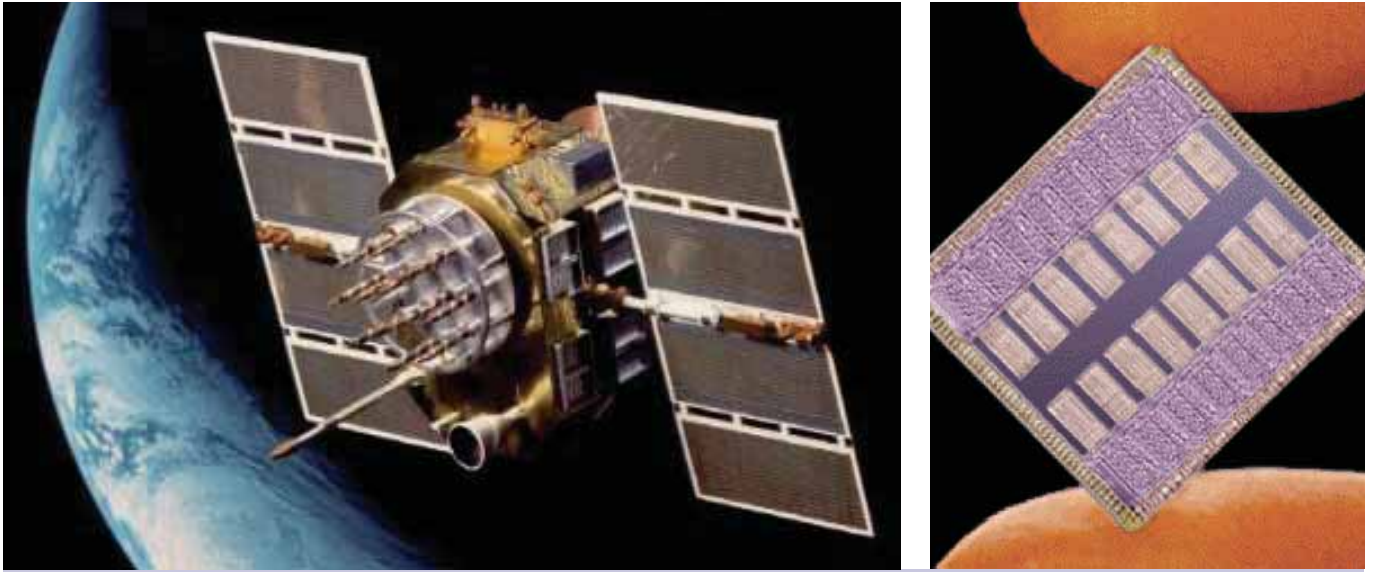
Left: Satellite-based global positioning systems rely on general relativity for their pinpoint accuracy. Right: The humble transistor - a quantum machine at the heart of all modern electronic devices. We rely on quantum mechanics and relativity every day, yet the two theories remain to be reconciled.
