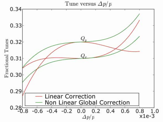
Figure 5: Horizontal and vertical chromaticity for Beam 2 after several correction option.
