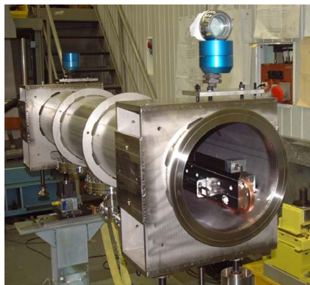
Figure 3: The TPSG6 diluter in its vacuum vessel.
