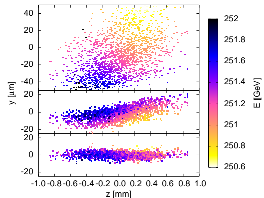
Figure 1: Example of tuning bumps in the ILC linac. The beam is plotted in the z - y plane, with color corresponding to energy, for different correction methods. Top plot shows beam after one-to-one correction. Middle plot shows the beam after Dispersion Free Steering (DFS), while the bottom plot shows the beam after DFS and optimization of emittance tuning bumps.
