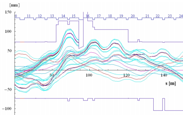
Figure 4: Superposition of horizontal beam envelope for the five islands at extraction. The numbers in the upper part identify the main magnets.
