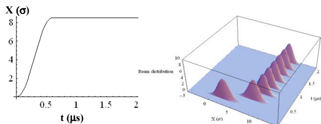
Figure 5: Kick time-dependence (left) and longitudinal and horizontal beam distribution (right) used in the analytical computations of the total beam losses for the MTE.
