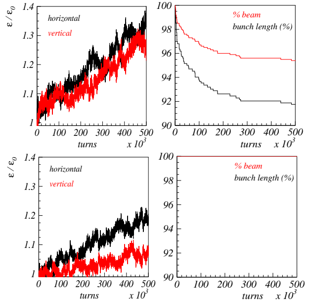
Figure 6: Simulations for SPS with different working point. Top: (26.18, 26.15), Bottom: (26.15, 26.18)
