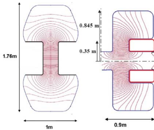
Figure 3: The test cavity (left) and the ideal 88 MHz cavity (right) compared. The ratio between peak field and gradient is preserved.
