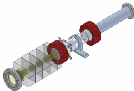
Figure 3: Test module for insertion in ESA beamline showing: low-Z absorber, Beamcal, FB BPM, material model of QFEX1. The total length is 50 inches.
