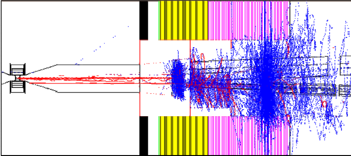
Figure 1: Example simulation of e+e- pairs produced via the beam-beam interaction and tracked through the material model of the IR. Secondary pairs (red lines) and photons (blue lines) are produced in EM showers originating at the mask and at the front face of QFEX1.
