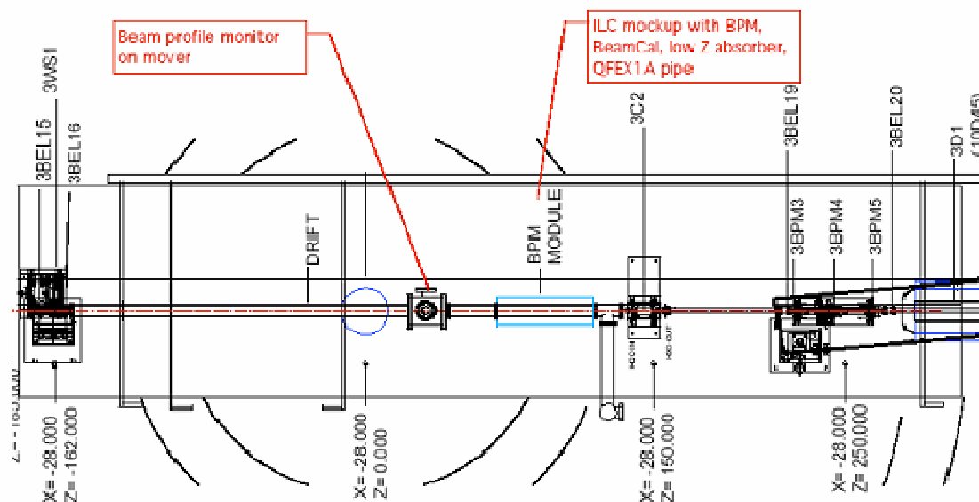
Figure 4: Proposed location for the FONT test module.
