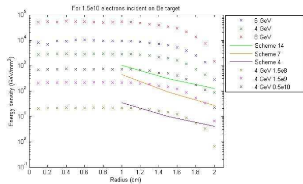
Figure 2: Spray beam energy density vs. radius from beamline centre in ESA (points), compared with corresponding ILC pair energy density (lines) for parameter schemes 4,7,14 that span the range of expected energy densities.
