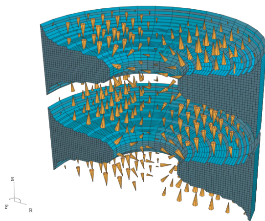
Figure 1. Electric fields within the FNAL cavity
