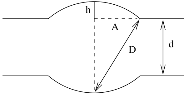
Figure 1: Schematic layout of the confocal resonator inserted into the CTF3 vacuum pipe. In the present design, the height of the CTF3 vacuum chamber is d = 3.7 cm. Furthermore, since we consider a confocal resonator, the distance D between the mirrors is equal to their radius of curvature R .
