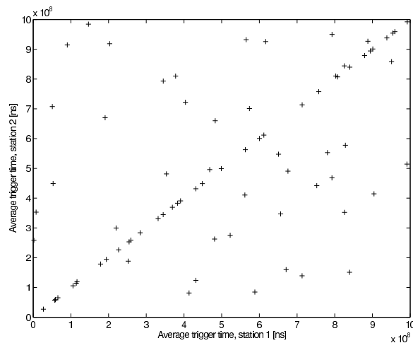
Figure 2. The trigger time for station 2 versus station 1 for events coinciding within the second. Out of 78 triggers, 33 coincided within 1 \mu s . The acquisition time was 120 hours.
