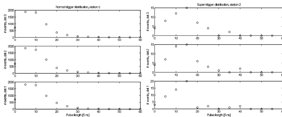
Figure 3. Pulse length distribution for ordinary triggers and super triggers in units of 5 ns for station triggers (left) and super triggers (right). A shift in pulse length is evident for the super triggers compared to the pulse length for the station triggers, indicating that super triggers originate from larger showers than station triggers.
