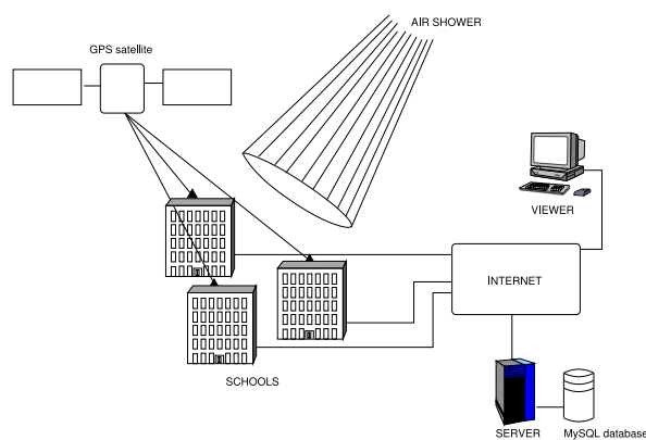
Figure 1. An overview of the SEASA system. The data flow is as follows: when an air shower triggers a station, a time stamp is provided by the GPS system and information about the event is sent over the internet to a central server. The server stores the data in a database and sends it to all active viewer clients.
