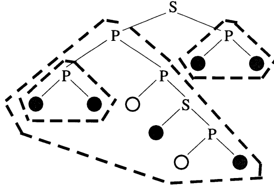
Figure 4-1: Three umbrellas of accesses to a location l . In this parse tree, each shaded leaf represents a thread that accesses l . Each umbrella of accesses to l is enclosed by a dashed line.
