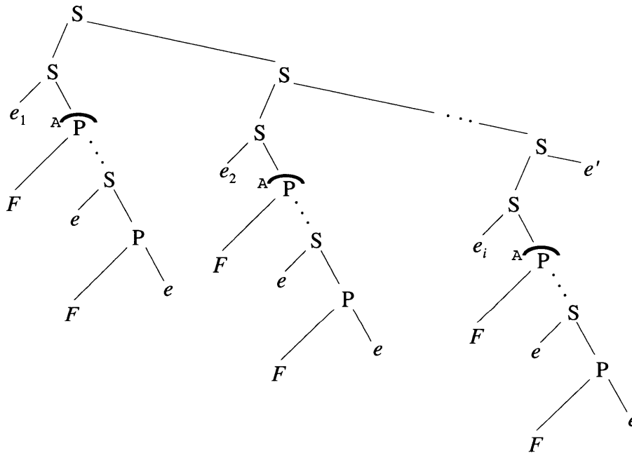
Figure 3-4: The SP-tree, with locked P-nodes, representing the generalized form of a critical section, protected by a single lock A . Although the lock is held across this entire tree, the P-nodes corresponding to the first spawns in each sync block are shown as locked P-nodes, as if separate instance of A were held across them. Also, the first threads of each sync block, e_1, e_2, \dots, e_i , and the thread at the end of the critical section, e' —none of which are descendants of a locked P-node—are considered to hold their own instances of A (not shown).
