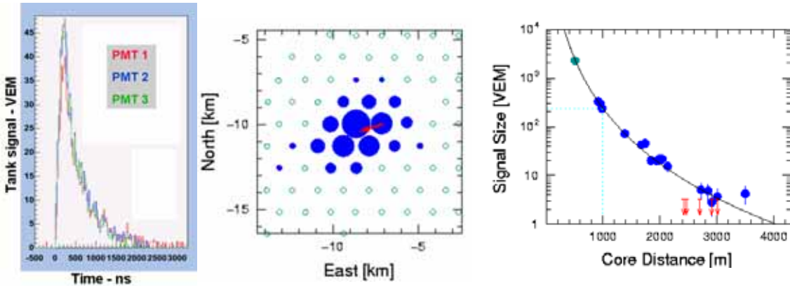
Figure 6. An example of a surface array event with an energy of 70 EeV and zenith angle of 48°. On the left is a typical FADC trace from one of the triggered stations located 1 km from the core. In the center is the hit pattern on the array with the axes in kilometers. On the right is the lateral density distribution of the event. The arrows correspond to stations that did not contribute to the trigger. The dotted line indicates the signal size at 1000 m or S(1000).
