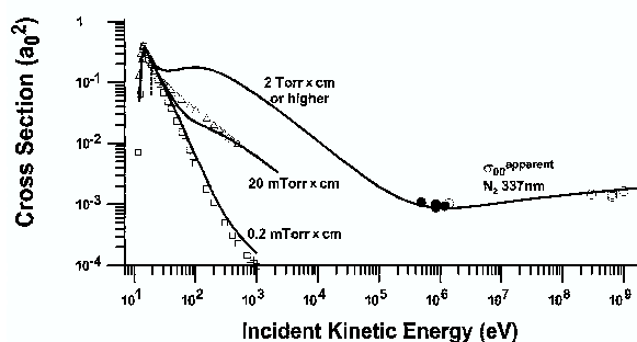
Figure 2. Apparent optical cross section \sigma_{00}^{ap} for 2P system of N_2 versus electron energy as predicted by the model of ref. [6] for several NR values (continuous lines). Data deduced from measurements of Nagano et al. (●) and Kakimoto et al. (○) at high pressure are in good agreement with the model. This model also accounts for experimental results at low pressure ( \Delta , \square ). See [6] for more details.
