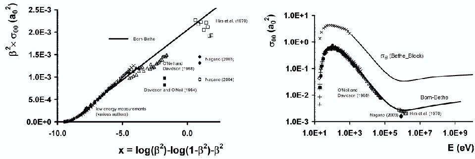
Figure 1. Optical cross section \sigma_{00} of the 1N system. Left: Available experimental data in a Fano plot together with a Born-Bethe fit. Right: Optical cross section versus electron energy. The Bethe Block function is shown for comparison.
