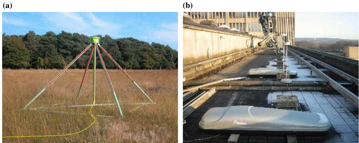
Figure 1. (a) LORUN prototype antenna: two (crossed) inverted-v-shaped dipoles in the legs of the PVC structure connected to two low-noise amplifier (LNA) located in the top box. (b) NAHSA particle detectors: scintillator plates connected to a photo multiplier tube (PMT) accommodated in ski-boxes on top of the building of the Radboud University Nijmegen.
