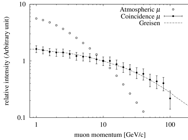
Figure 3. EAS muon momentum spectrum. The solid circles: the muon flux associated with EAS. The open circles: the atmospheric muon flux. The dashed curve indicate the calculated flux using Greisen's equation (1).
