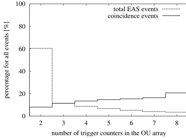
Figure 2. The distributions of the number of trigger counters in the OU array. The dashed histogram: for all EAS events in the OU array. The solid histogram: for coincidence events between the OU array and the Okayama telescope.
