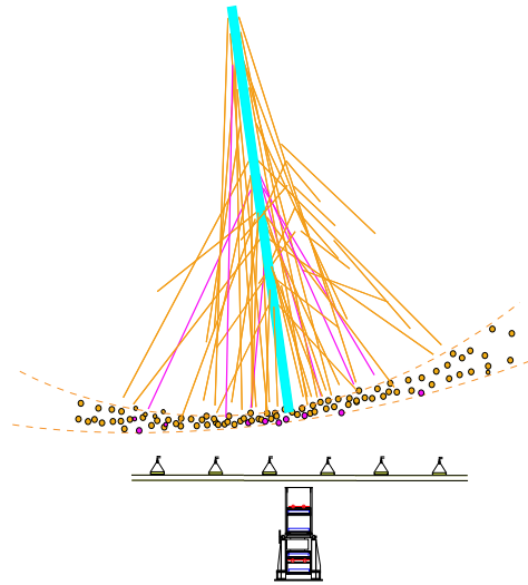
Figure 1. The arrangement of detectors, the OU array and the Okayama telescope. An EAS event comes in both detectors within \pm 1\mu sec, EAS signal is recorded by the telescope.
