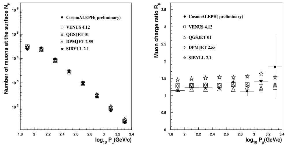
Figure 2. Number of vertical muons at the surface and their charge ratio compared with MC simulations based on different hadronic interaction models.
