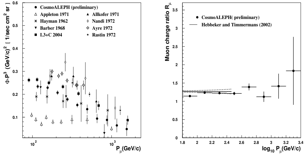
Figure 1. Momentum spectrum and charge ratio for vertical muons compared with other experiments[5, 18].
