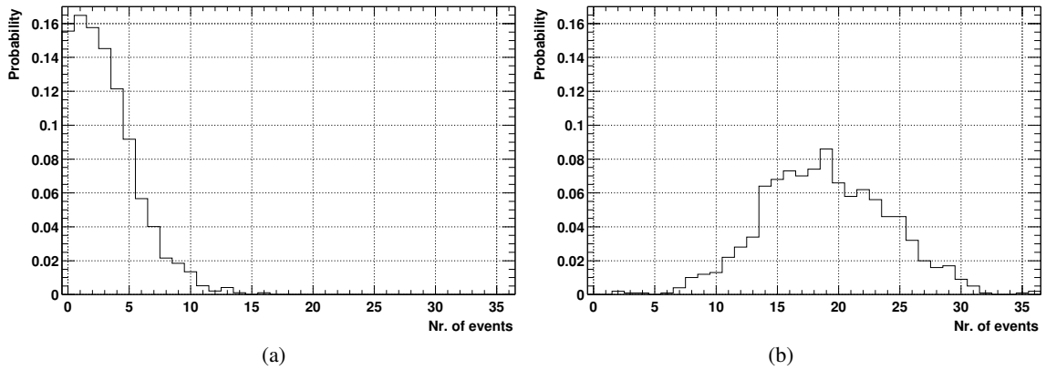
Figure 1. Probability density function for two different signal contributions. (a) : 2.0 \cdot 10^{-7} \text{GeV cm}^{-2} \text{s}^{-1} \text{sr}^{-1} , (b) : 10^{-6} \text{GeV cm}^{-2} \text{s}^{-1} \text{sr}^{-1} .
