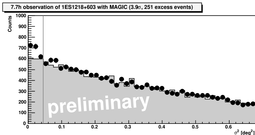
Figure 1. \theta^2 plot for 7.7 h of 1ES1218+603 data at zenith angles < 12^\circ after cuts as described in [9]. The off-data used is shown gray shaded, it was scaled by the inetgral between 0.2deg^2 and 0.5deg^2 with a factor 1.13. The Li/Ma-significance and the number of excess events was calculated from the data below 0.045deg^2 (marked by a gray vertical line). The on-data is shown with full dots.
