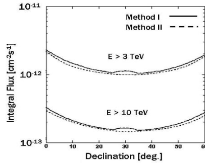
Figure 3 Declination dependence of 90% C.L. upper limits.
