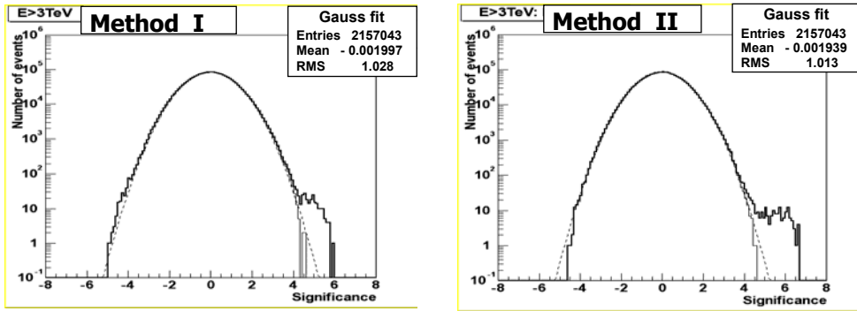
Figure 1 Significance distributions of all directions on the sky map from Method I and Method II. Solid lines in both figures are derived from all cells defined in analyses. Histograms of thin lines excludes those cells, centers of which have distances to Crab or Mrk421 of shorter than 2^\circ . The dashed histogram represents the normal Gaussian distribution.
