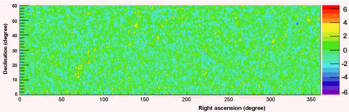
Figure 2. Map of significance distribution by Tibet III (1999~2004) given by Method I. Window size of each bin is of radius 0.9degree. Two directions with significance greater than 5 sigma are Crab (left) and Mrk421(right).
