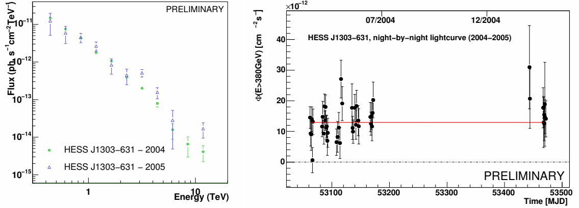
Figure 2. Left: The differential energy spectrum of HESS J1303-631 in 2004 and 2005. The two data sets are in good agreement. Right: The HESS J1303-631 light curve from February 2004 until March 2005. Shown is the integral flux \Phi(E > 380 \text{ GeV}) vs. time in night-by-night bins. The fit of a constant function to data (solid line) results in a \chi^2/\text{d.o.f.} of 41/45 being compatible with constant emission.
