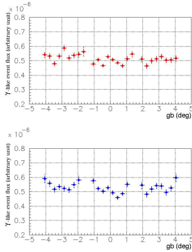
Figure 2. Latitude profile of gamma-ray like events for l = -19^\circ.5 region. Upper:T2-T3, Lower:T2-T4.
