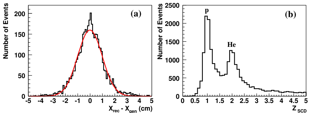
Figure 2. Results of CAL trajectory reconstruction, (a) difference between the measured position and the actual incident position at the SCD, from electron simulation, (b) preliminary SCD charge distribution for hydrogen and helium from the first CREAM flight.
