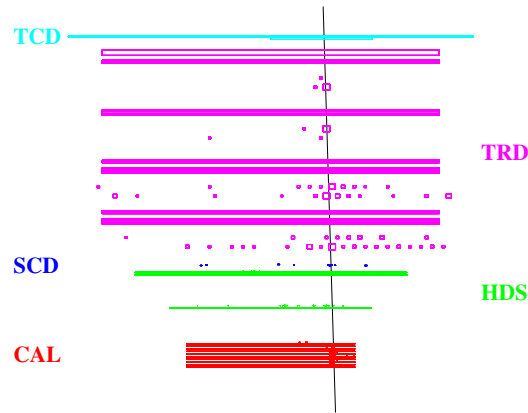
Figure 3. CREAM event display shows each sub-detector's responses to a high energy carbon candidate, along which a trajectory is reconstructed. Box size is proportional to the corresponding signal size.
