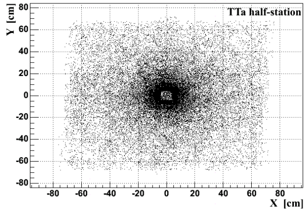
Figure 10: The distribution of hits in TTa.
