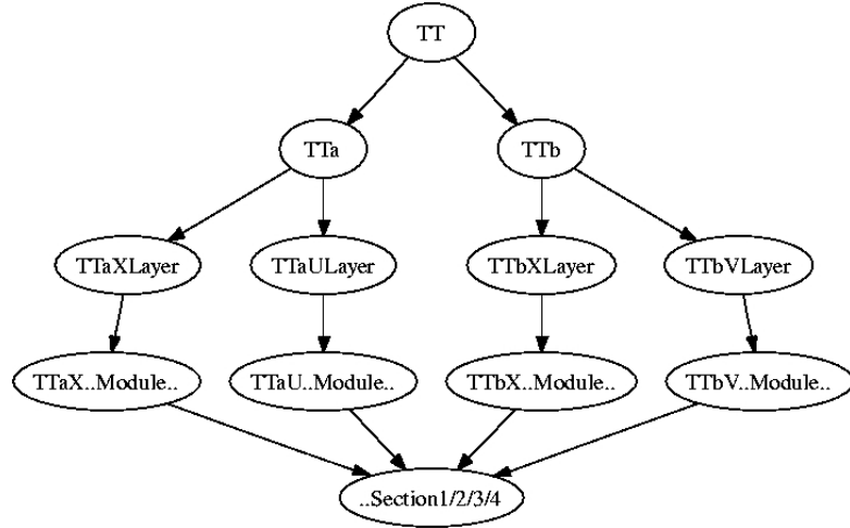
Figure 8: A tree of the detector elements for TT station.
