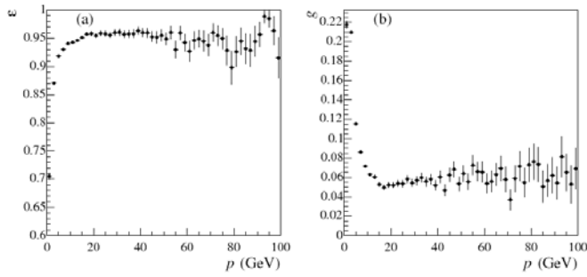
Figure 8. The tracking efficiency and ghost rate for long tracks.
