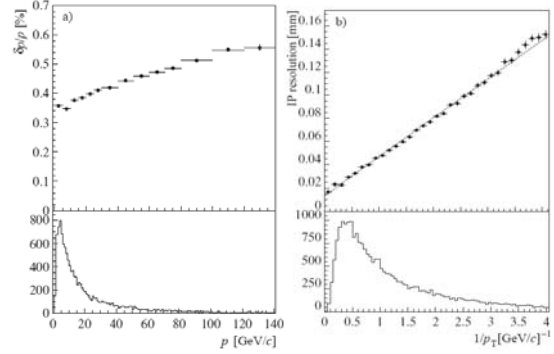
Figure 10. The momentum (a) and impact parameter (b) resolution for B-decay tracks. B-decay tracks are generally long tracks. The histograms at the bottom of the plots show the momentum and IP distribution of B-tracks.
