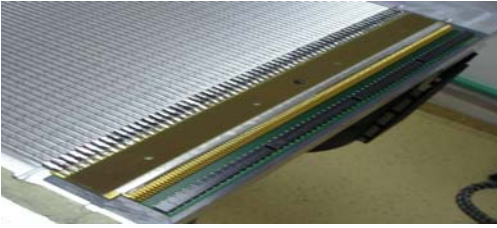
Figure 5. One of the straw tube chambers while it is being assembled. Two layers of straws are visible in the picture.
