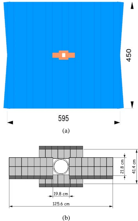
Figure 6. The layout of one of the three tracking stations. The center region is covered by a silicon strip detector (b) which is surrounding the beam pipe. The outer region (a) is covered by a straw tube detector (the dimensions are given in cm).
