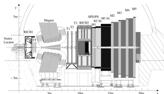
Figure 1. Schematic view of the LHCb detector.
