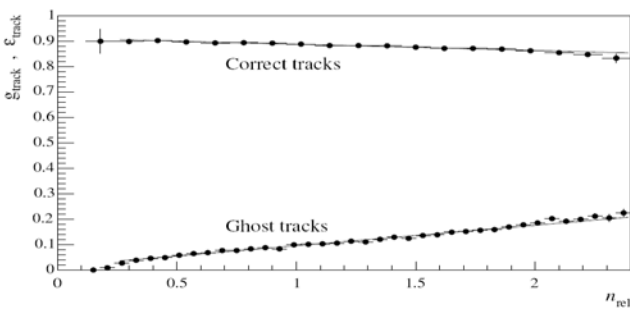
Figure 9. The tracking efficiency and the ghost rate for long tracks as a function of the relative hit multiplicity, i.e. the hit multiplicity of the tracking detectors divided by the average hit multiplicity.
