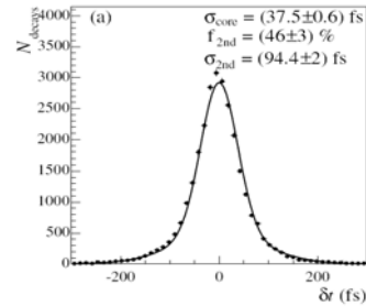
Figure 11. A double Gaussian fit of the decay time resolution for B_s -mesons which decay as B_s \rightarrow D_s K .
