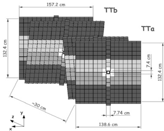
Figure 3. A schematic layout of the Trigger Tracker. The square elements represent the silicon sensors, which have a size of 9.44 \times 9.64 cm 2 .
