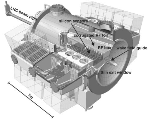
Figure 2. Schematic view of the Velo detector. The corrugated foil separates the beam and detector vacuum, and serves as an RF shield for the detector modules.
