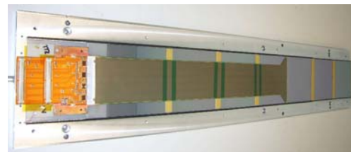
Figure 4. One of the TT modules. There are four sensors connected to one front-end hybrid. The long kapton cable serves to connect the inner three sensors to their readout hybrid, which is located outside the detector acceptance.
