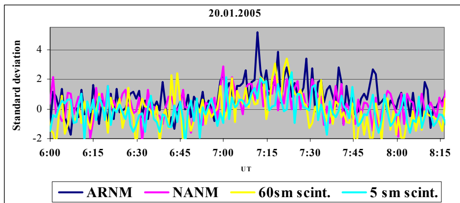
Figure 1. Multiple detection of GLE by ASEC monitors
