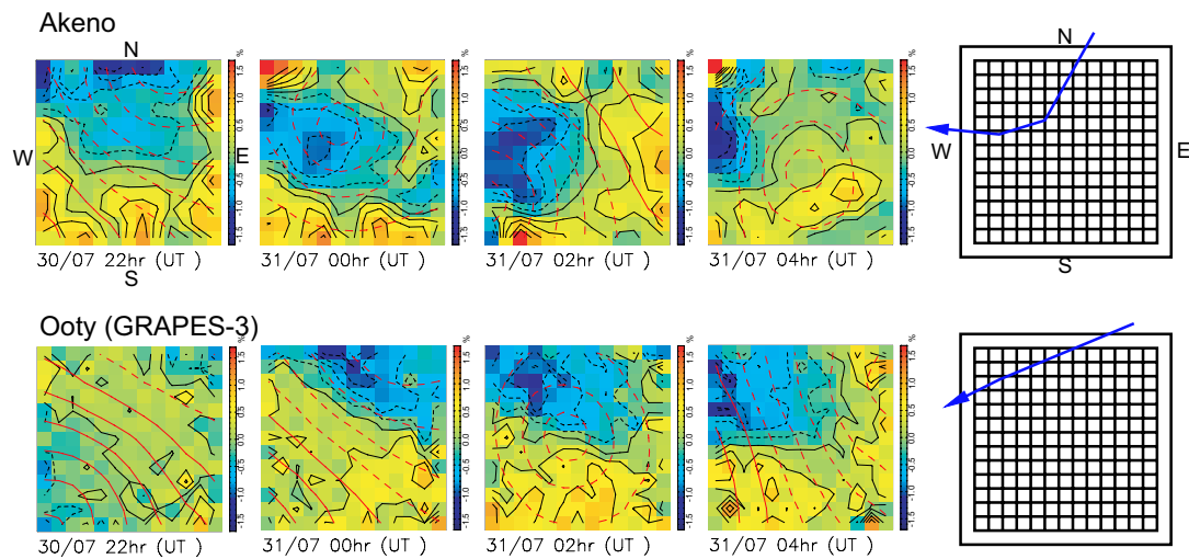
Figure 4. Intensity map in FOV of Akeno and Grapes-3 muon telescopes. Right panel shows path of deficit cone in FOV of each telescope.
