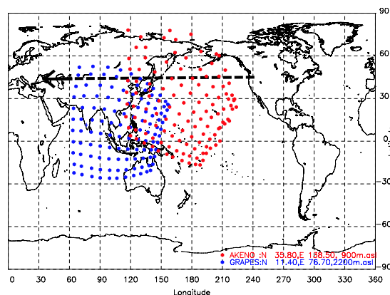
Figure 2. Observed directions of 2 muon telescopes.
