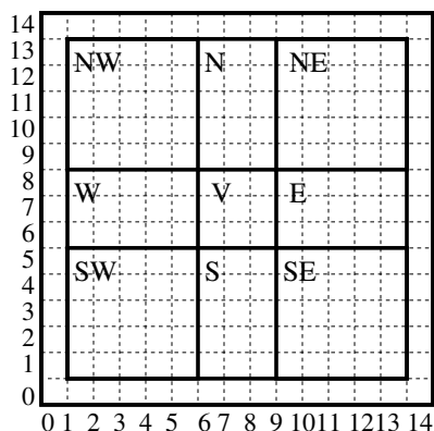
Figure 1. 15 \times 15 cells in the FOV.
