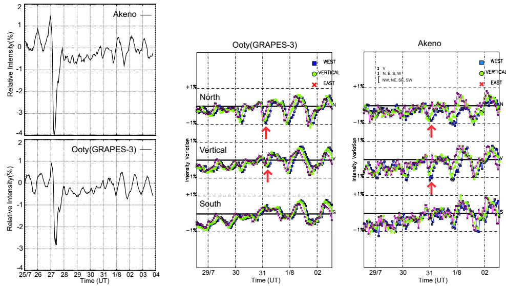
Figure 3. Relative muon intensity at Akeno and Grapes-3 muon telescopes. Left: Variation in muon rate observed at GRAPES-3 and Akeno are shown. Statistical errors in GRAPES and Akeno are 0.036% and 0.01% respectively. Center: Variation in 9 direction at GRAPES-3 are shown. Statistical error for each series is 0.09% to 0.15%. Right: Variation in 9 direction at Akeno are shown. Statistical error for each series is 0.018% to 0.029%.
