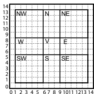
Figure 1. 15 \times 15 cells in FOV. The FOV was reconfigured into 9 (NW,N,NE,W,V,E,SW,S,SE) also for this analysis.
