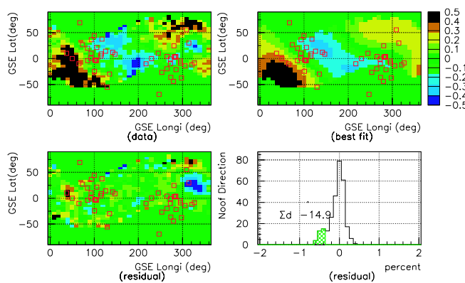
Figure 4. An example of subtraction of background anisotropy. (2001/3/25-26)
