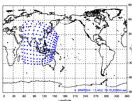
Figure 2. Asymptotic Viewing direction at the median rigidity of muon telescope in geographical coordinate
