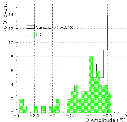
Figure 3. Distribution of the amplitude of observed Forbush decreases
