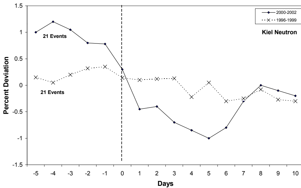
Figure 3. SSC associated high speed solar wind streams superposed with cosmic ray intensity.
