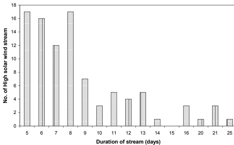
Figure 1. The time duration of high speed solar wind streams for the period of 1996 to 2002.
